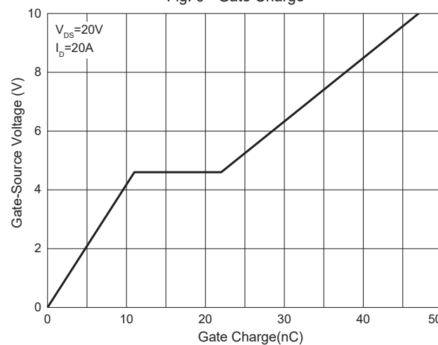
Fig. 6 - Gate Charge
