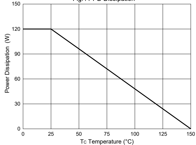
Fig.11-PD Dissipation
