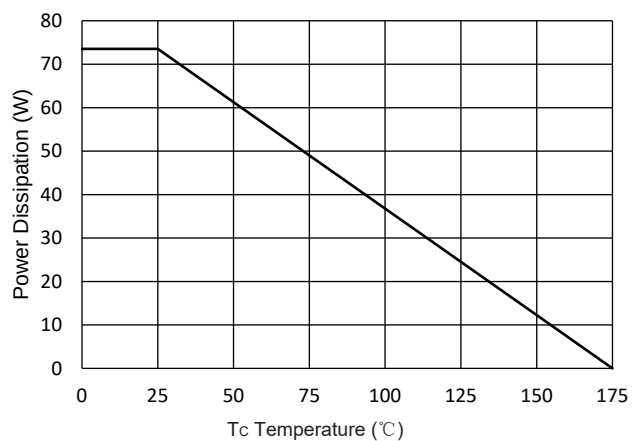
Fig.11 Power Dissipation
