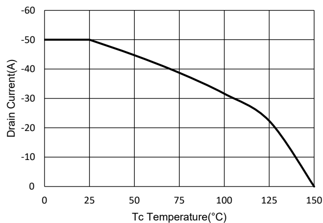
Fig.10 Drain Current
