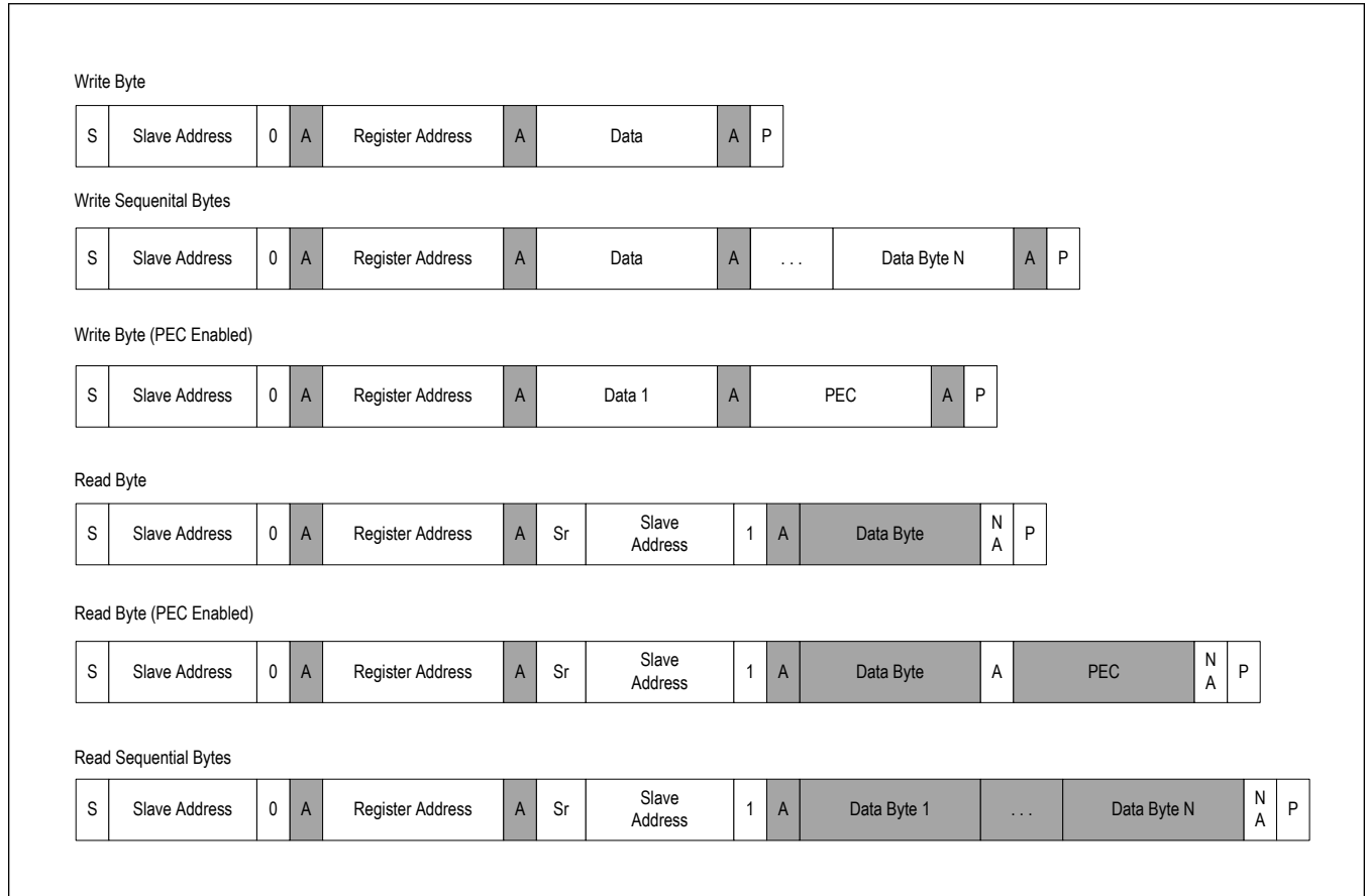
Figure 8. Data Format of I 2 C Interface
