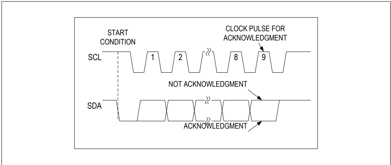
Figure 7. Acknowledge Condition
