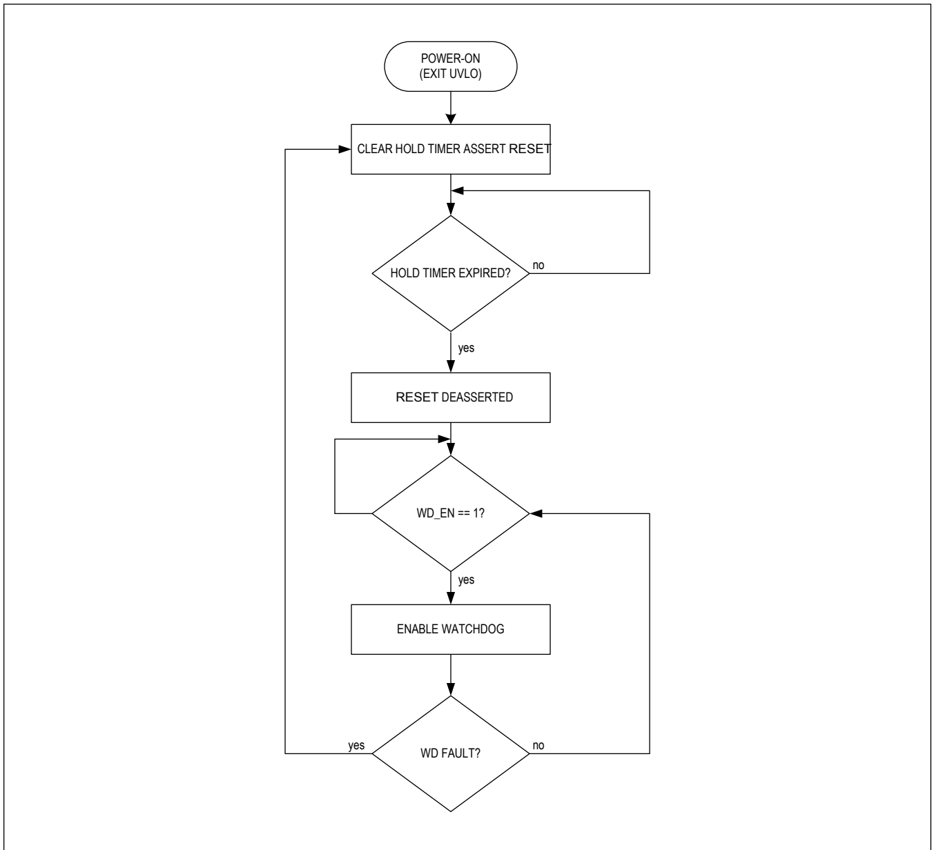
Figure 1. Watchdog Control
