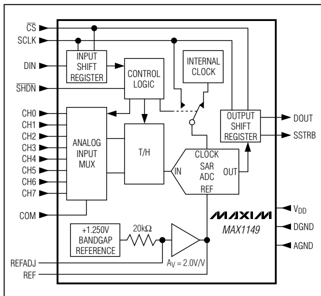
Figure 5. Functional Diagram
