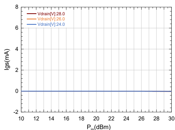
Gate Current over Voltage vs. P_{IN}
