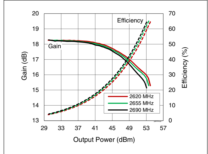
Figure 4. CW Performance
