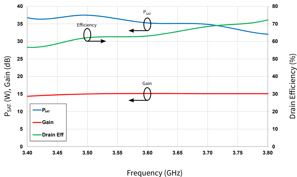
Figure 2. P_{SAT} , Gain, and Drain Efficiency vs Frequency of the CG2H40025F in the CG2H40025-AMP
