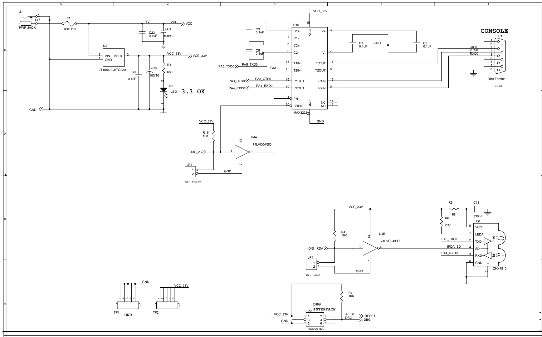
Figure 4. Schematic for Z8 Encore! XP F0822 Series Evaluation Board
