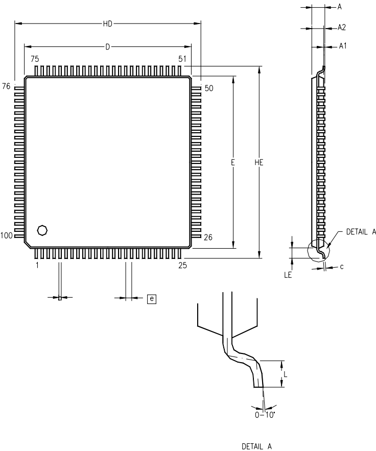
Figure 31. 100-Lead VQFP Package Diagram
