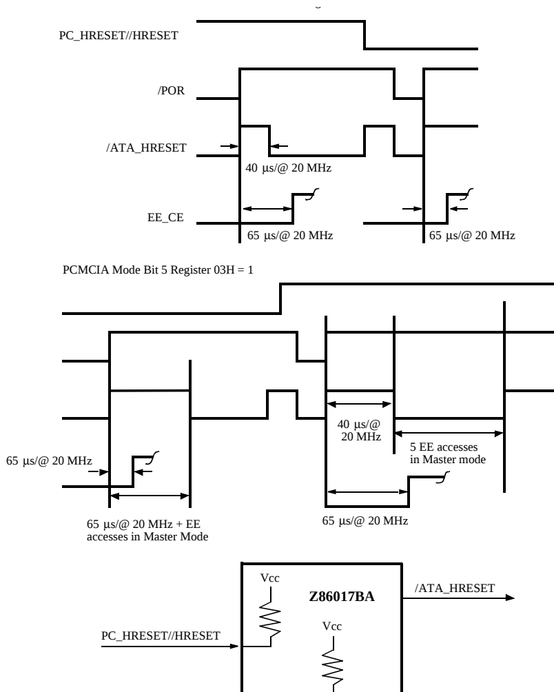
Figure 27. Z16017BA Reset Timing PCMCIA Mode
