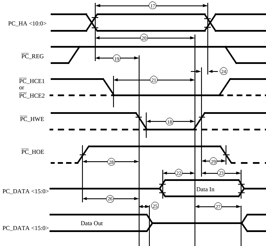
Figure 19. PCMCIA Write Memory Timing, No Wait States
