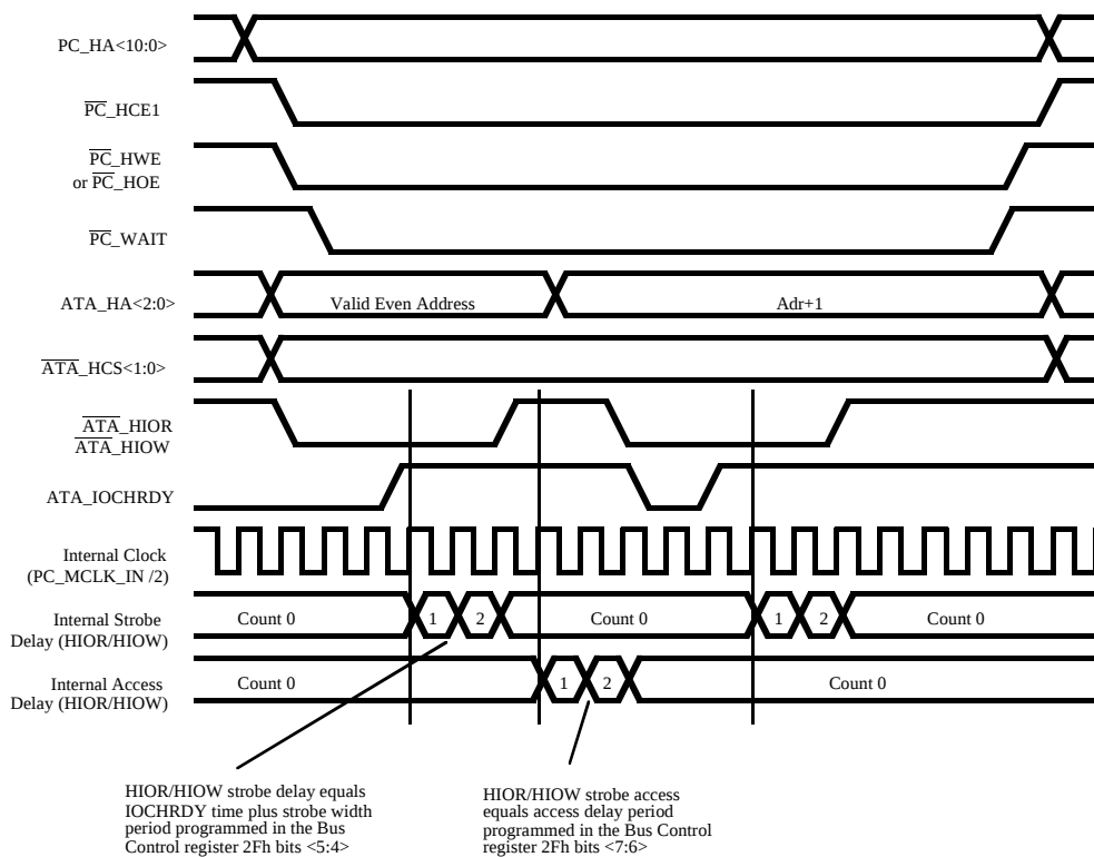
Figure 10. Word-to-Byte Timing
