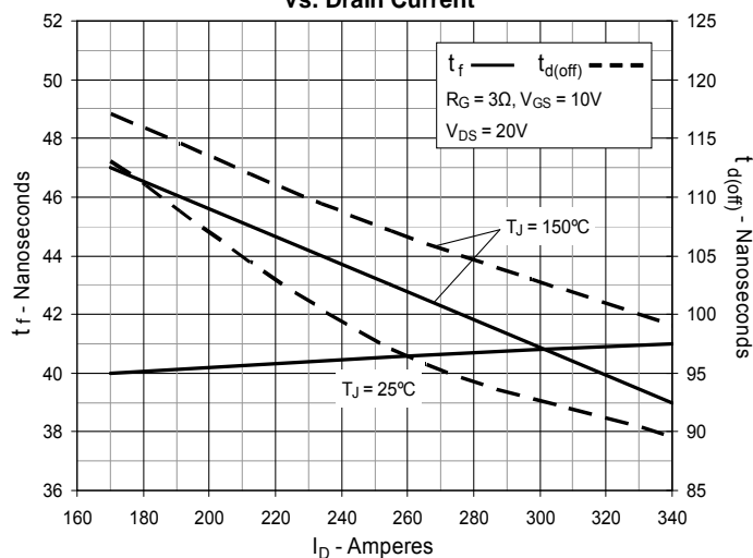
Fig. 17. Resistive Turn-off Switching Times vs. Drain Current
