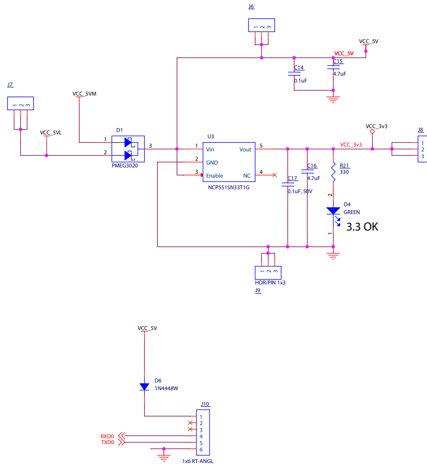
Figure 16. Z32F128 MCU Module Schematic, #2 of 2
