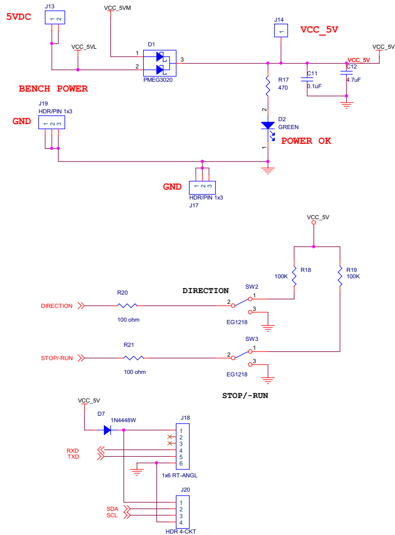
Figure 22. Z51F3220 MCU Module Schematic, #2 of 2
