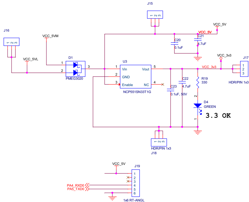
Figure 18. Z16FMC MCU Module Schematic, #2 of 2
