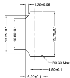
Reference Panel Cut Out Dimension
