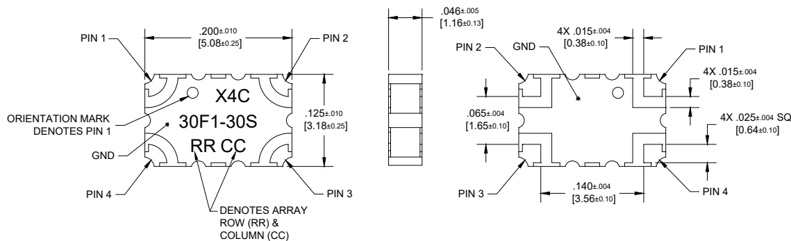
Dimensions are in Inches [Millimeters] X4C30F1-30S Mechanical Outline
