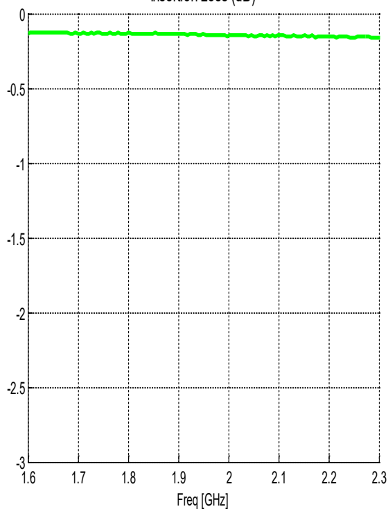
Insertion Loss (dB)
