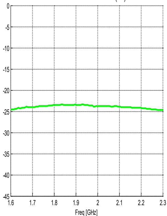
Return Loss at Isolated Port (dB)
