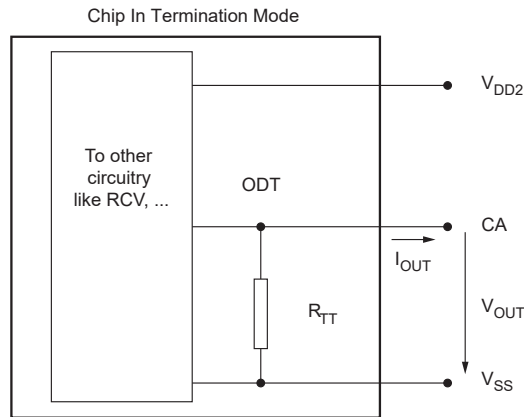
Figure 4.113a — On Die Termination for CA for LPDDR4
