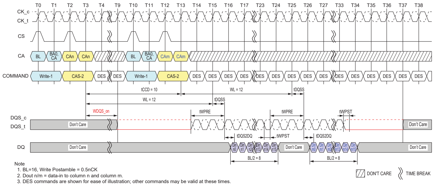
Figure 4.37 — Consecutive Writes Operation: t_{CCD} = \text{Min} + 2, 0.5n\text{CK} Postamble
