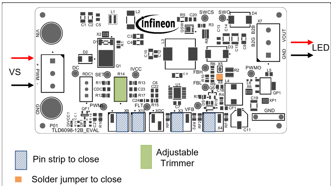
Figure 3 Current adjustment
