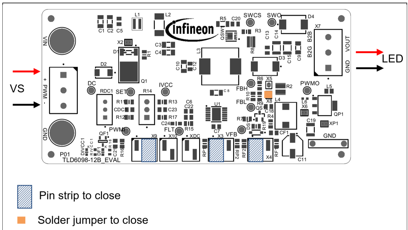
Figure 2 Default configuration of the board
