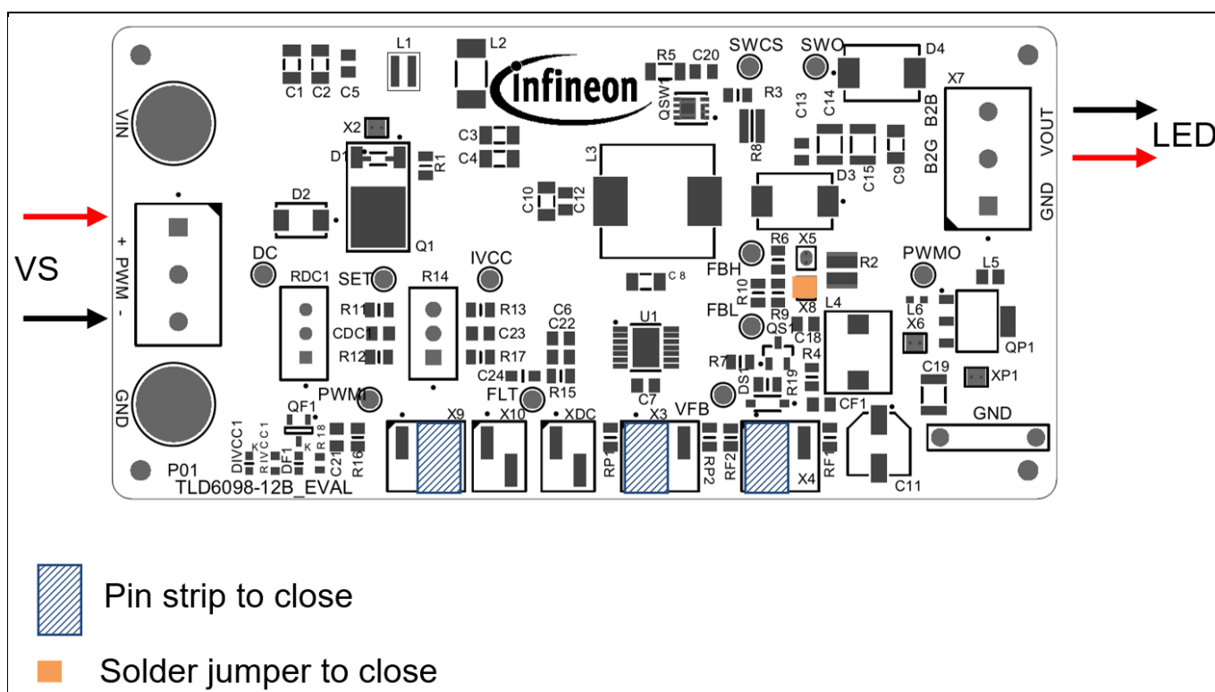
Figure 6 Boost to battery connection
