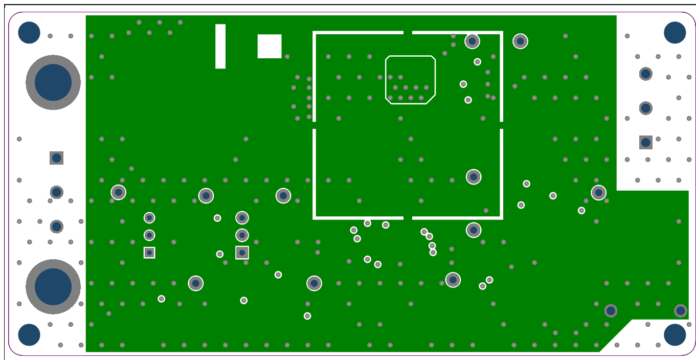
Figure 13 PCB layout internal 2
