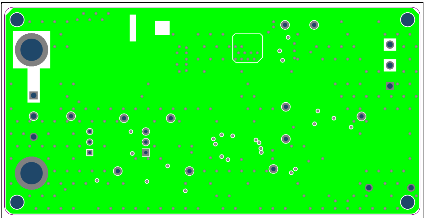
Figure 12 PCB layout internal 1
