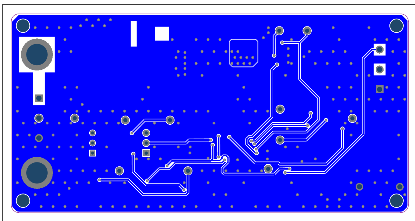
Figure 14 PCB layout bottom view
