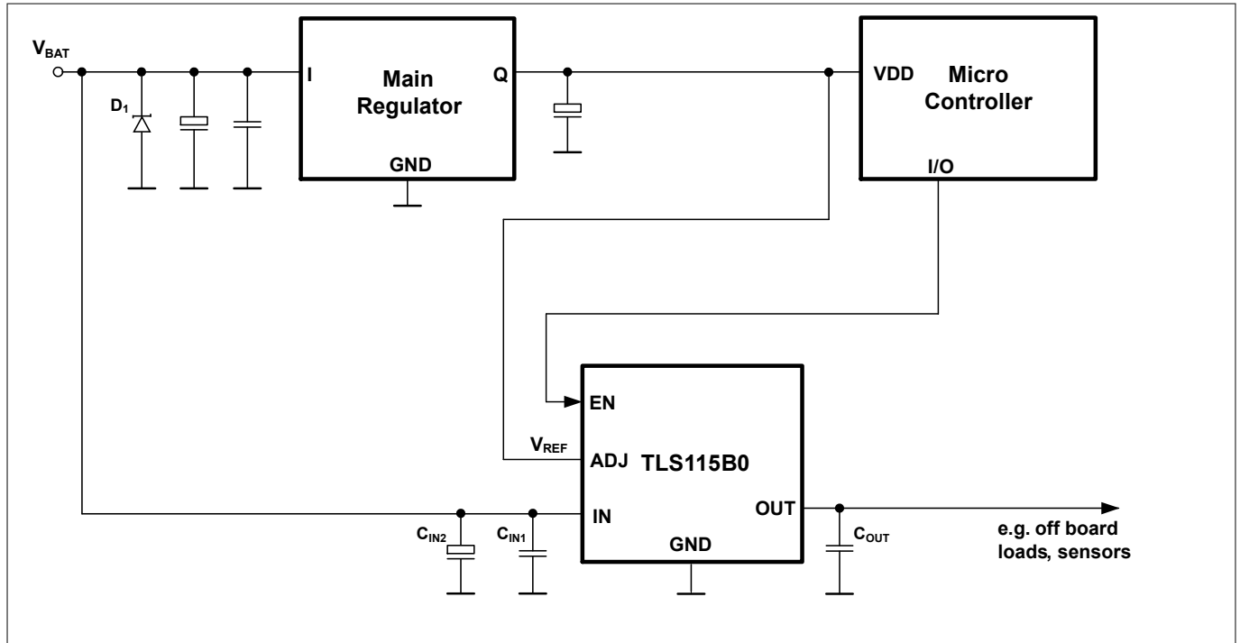
Figure 3 Application diagram
