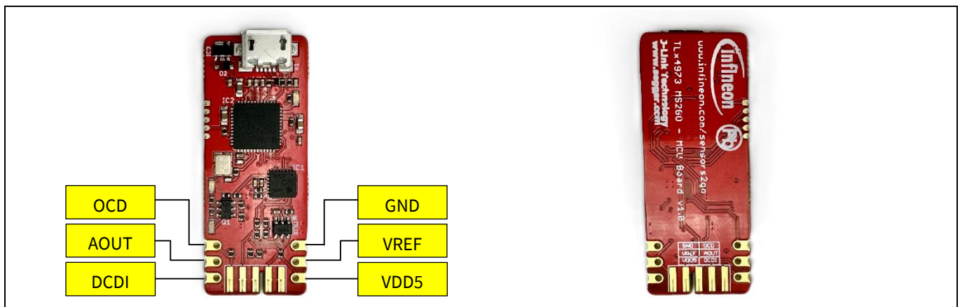
Figure 14 MCU Board Top and Bottom View
