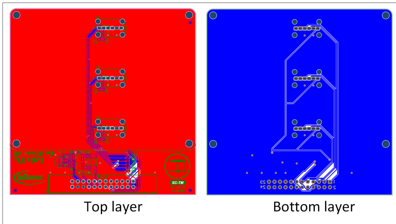
Figure 10 Evaluation board PCB layout (top and bottom layer)
