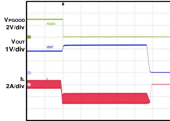
Over-Voltage Protection
