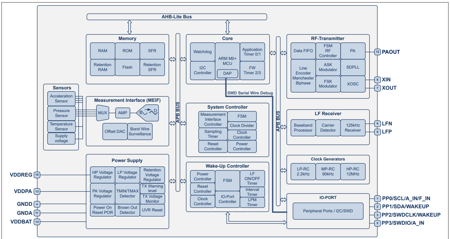
Figure 4 Block diagram
