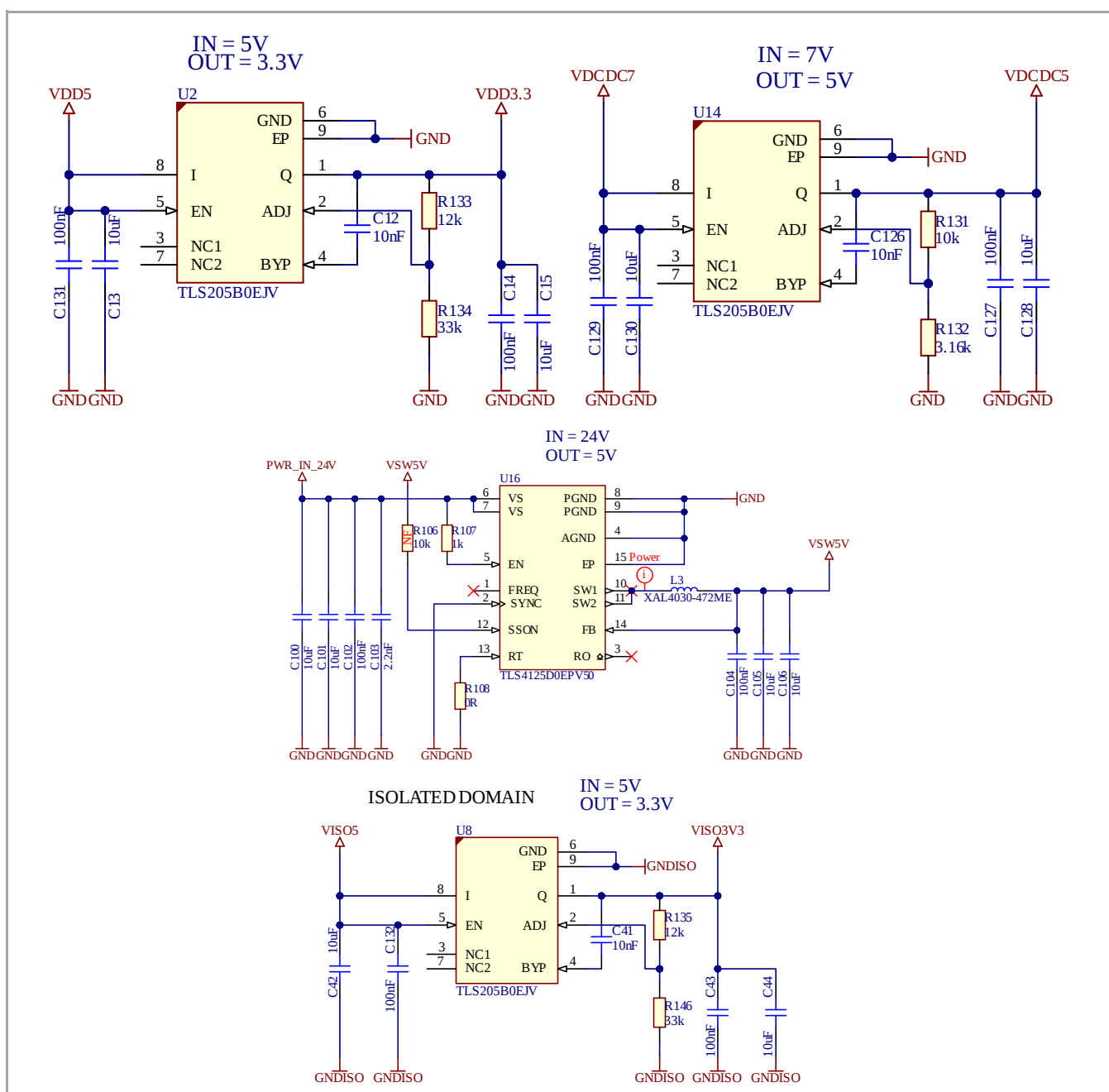
Figure 24 Voltage regulators
