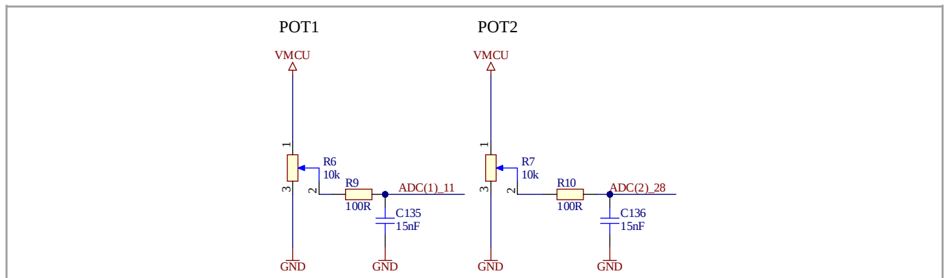
Figure 33 Potentiometers
