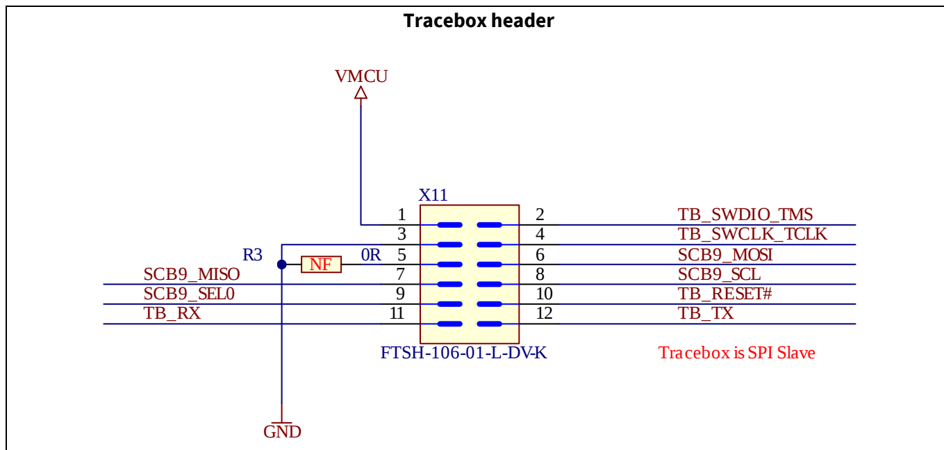
Figure 20 Tracebox header
