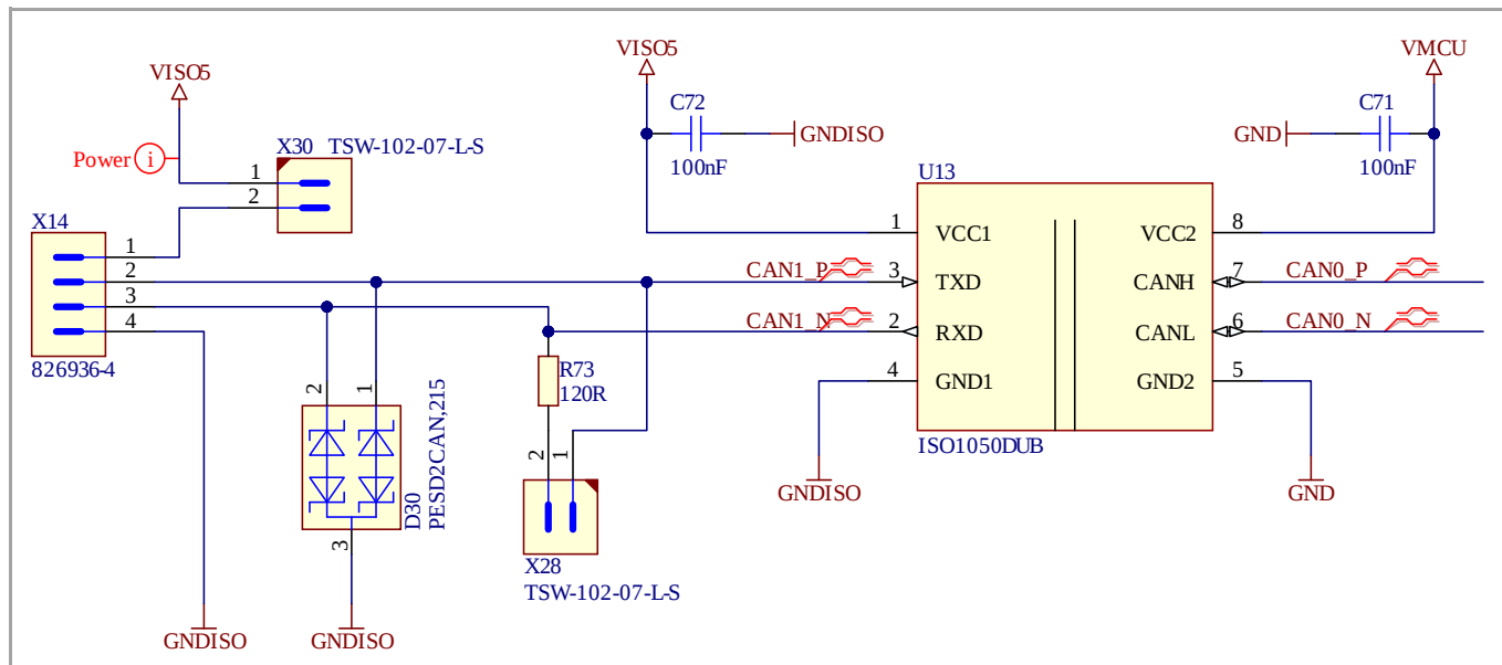
Figure 21 CAN interface and isolation
