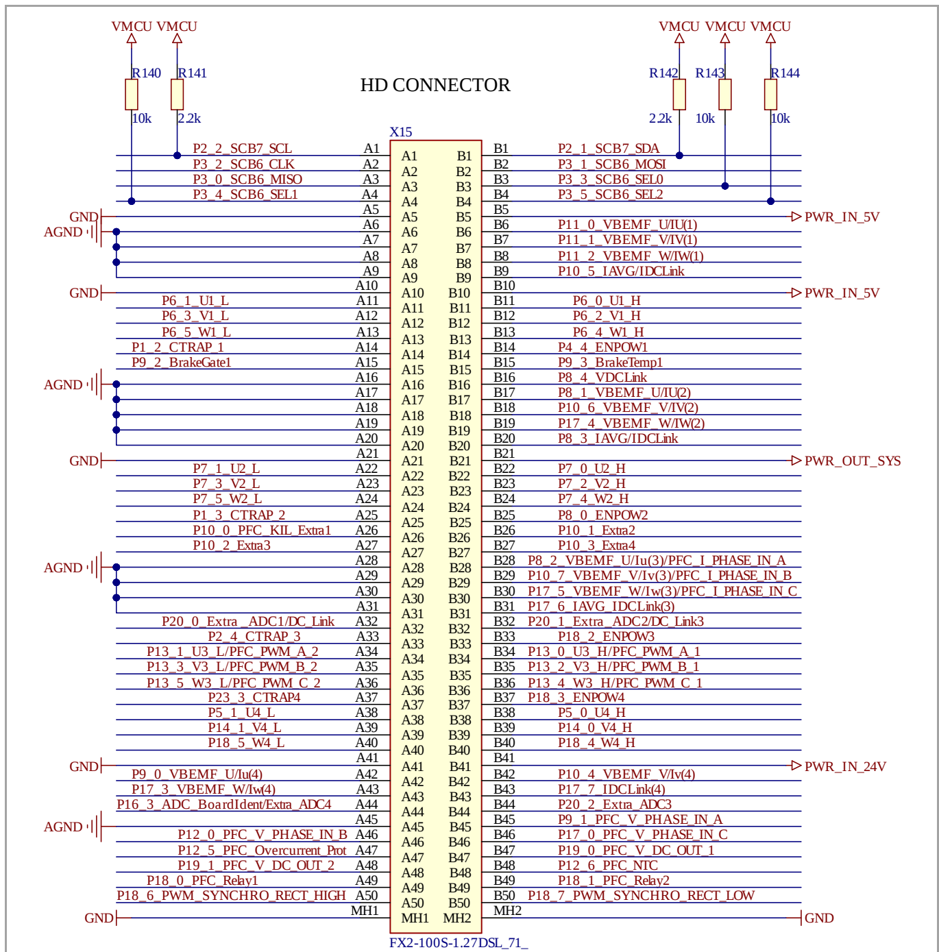
Figure 29 High-density connector
