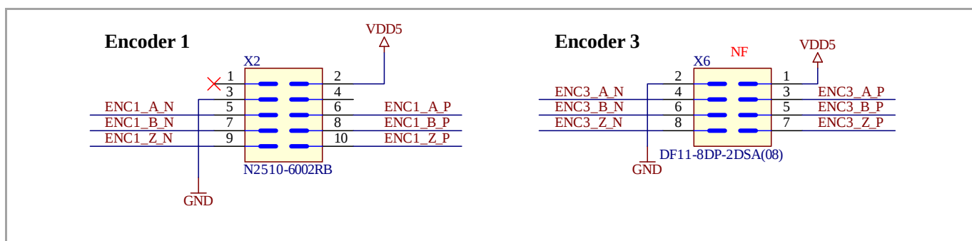
Figure 36 Encoder headers
