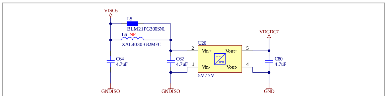
Figure 23 Power interconnection
