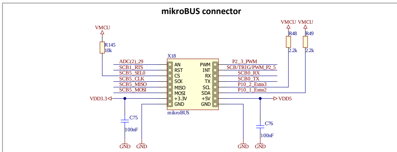
Figure 26 mikroBUS connector
