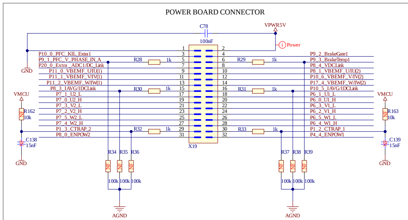
Figure 28 Power board connector
