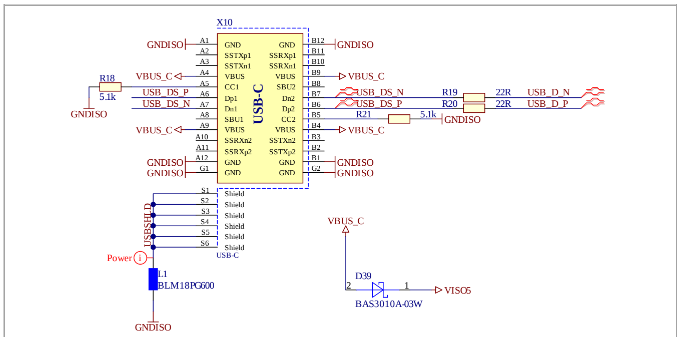
Figure 22 USB-C connector
