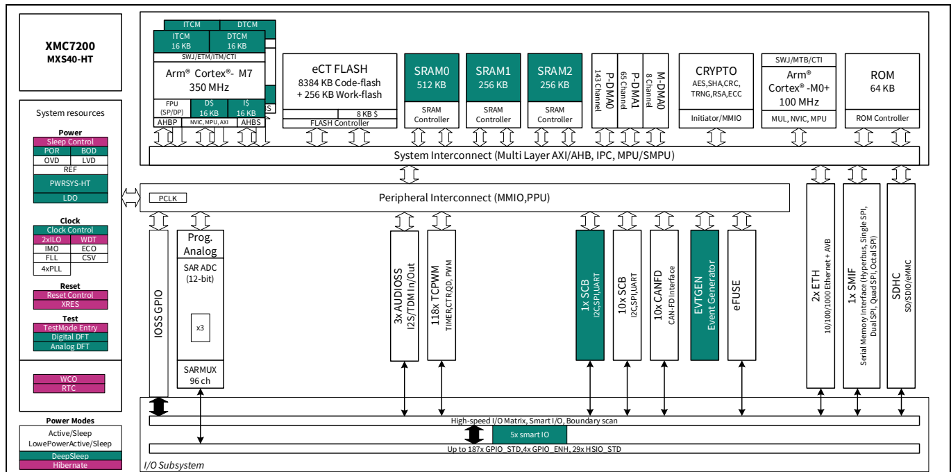
Figure 4 XMC7200D block diagram
