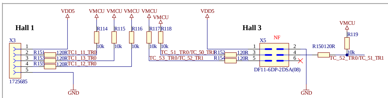
Figure 35 Hall headers
