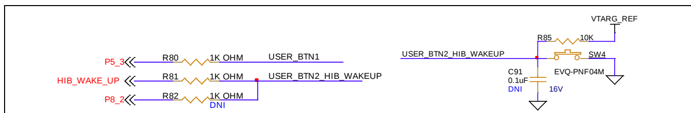
Figure 46 User buttons
