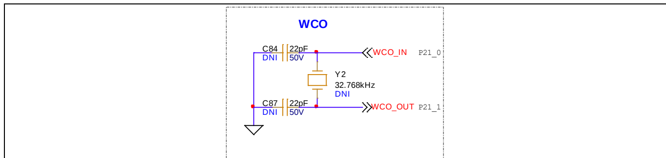
Figure 45 WCO
