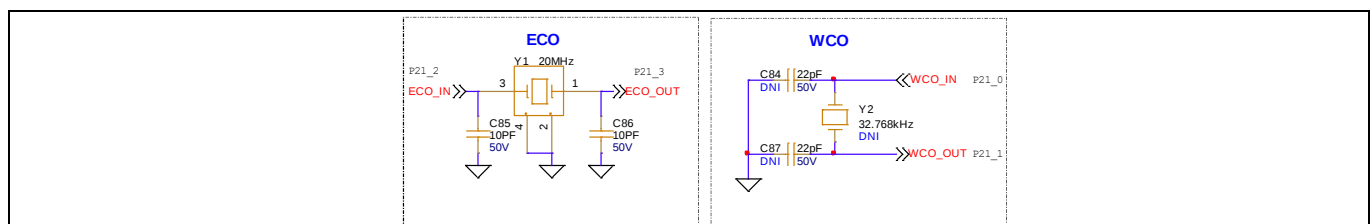
Figure 34 Crystal oscillators
