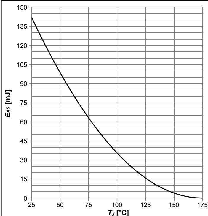
Diagram 13: Avalanche energy
