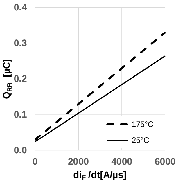
Figure 19 Typical reverse recovery charge as a function of diode current slope (Q_{rr} = f(di_i/dt), V_{DD} = 800V, V_{GS} = 0V/18V, I_D = 2A, \text{ind. load, test circuit in Fig.E, body diode at } V_{GS} = 0V)
