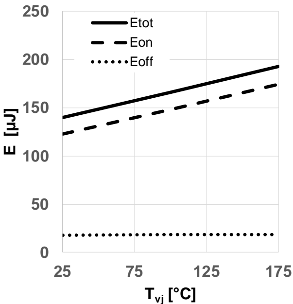
Figure 15 Typical switching energy losses as a function of junction temperature ( E = f(T_{vj}) , V_{DD} = 800V , V_{GS} = 0V/18V , R_{G,ext} = 2\Omega , I_D = 8.5A , ind. load, test circuit in Fig. E, diode: body diode at V_{GS} = 0V )
