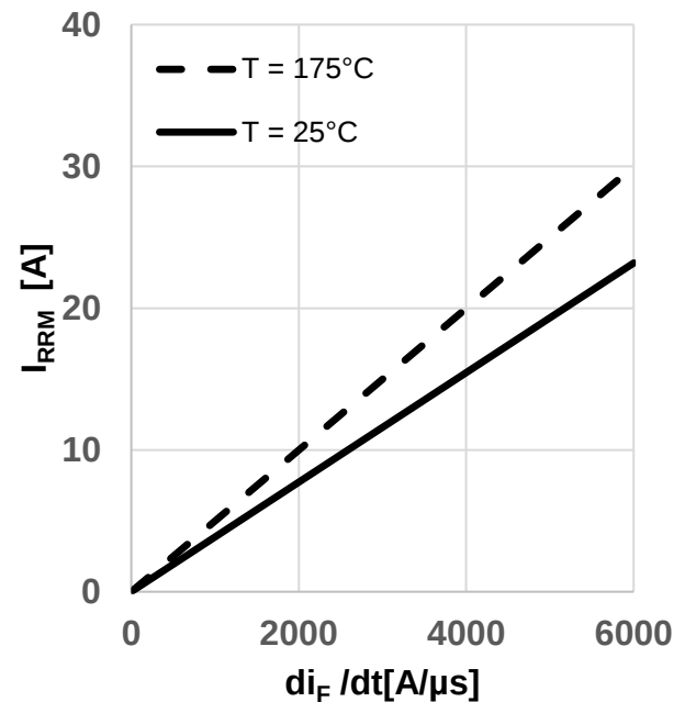
Figure 20 Typical reverse recovery current as a function of diode current slope (I_{rrm} = f(di_t/dt), V_{DD} = 800V, V_{GS} = 0V/18V, I_D = 16A, \text{ind. load, test circuit in Fig. E, body diode at } V_{GS} = 0V)
