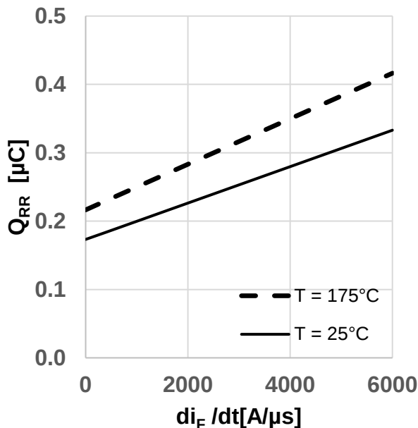
Figure 19 Typical reverse recovery charge as a function of diode current slope (Q_{rr} = f(di_t/dt), V_{DD} = 800V, V_{GS} = 0V/18V, I_D = 16A, \text{ind. load, test circuit in Fig. E, body diode at } V_{GS} = 0V)
