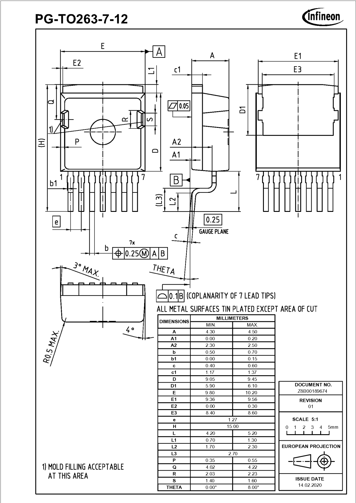
Figure 22 Package drawing
