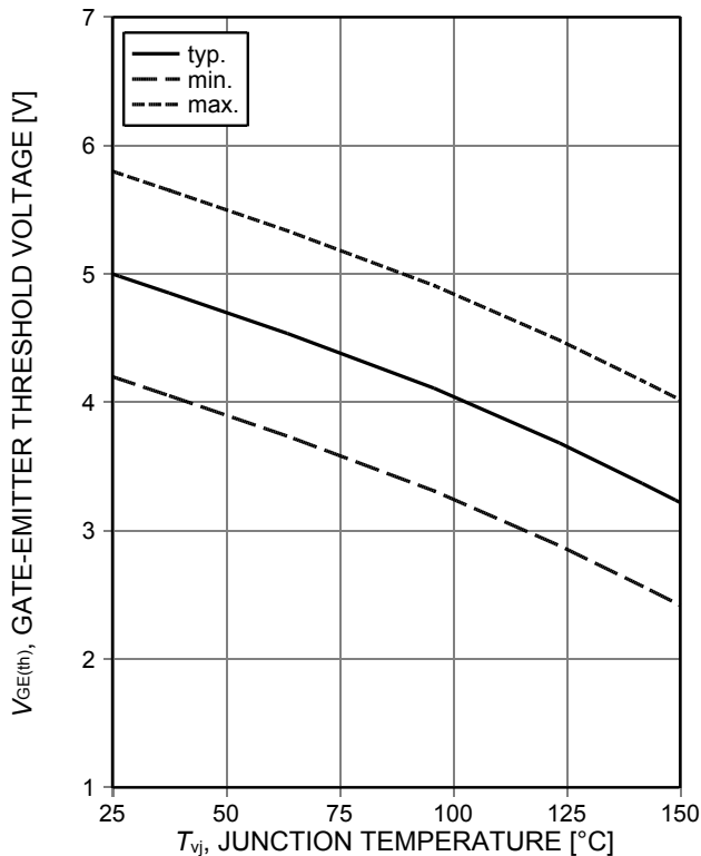
Figure 11. Gate-emitter threshold voltage as a function of junction temperature ( I_C=1mA )
