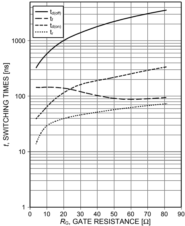
Figure 9. Typical switching times as a function of gate resistance (inductive load, T_{vj}=150^{\circ}C , V_{CE}=400V , V_{GE}=0/15V , I_C=75A , dynamic test circuit in Figure E)
