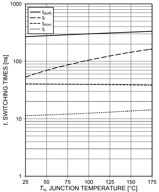
Figure 10. Typical switching times as a function of junction temperature (inductive load, V_{CE}=400V , V_{GE}=0/15V , I_C=75A , R_{G(on)}=4\Omega , R_{G(off)}=4\Omega , dynamic test circuit in Figure E)
