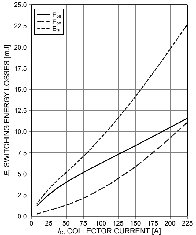
Figure 12. Typical switching energy losses as a function of collector current (inductive load, T_{vj}=150^{\circ}C , V_{CE}=400V , V_{GE}=0/15V , R_{G(on)}=4\Omega , R_{G(off)}=4\Omega , dynamic test circuit in Figure E)
