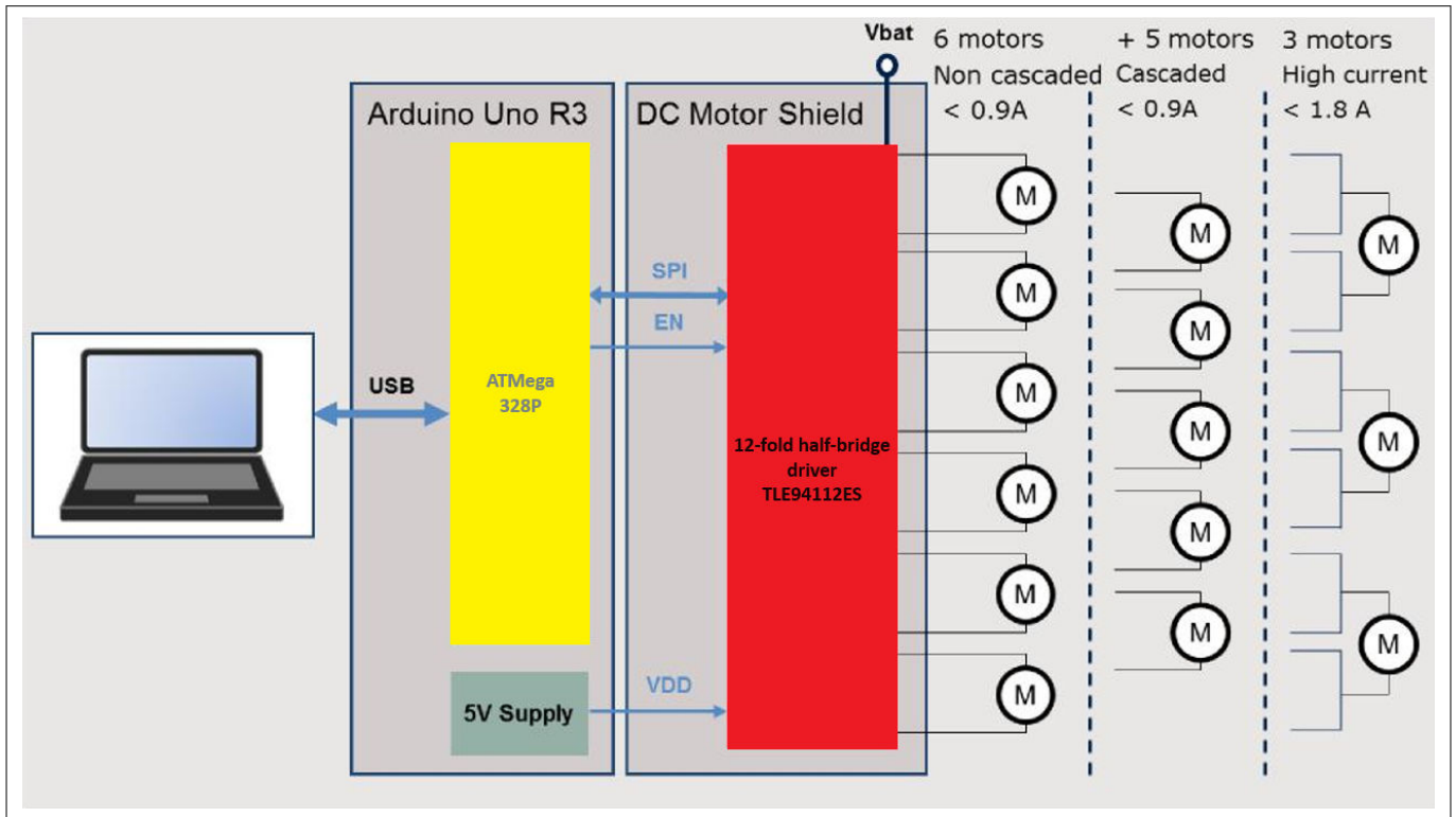
Figure 2 Simplified application diagram with TLE94112ES driving DC motors
