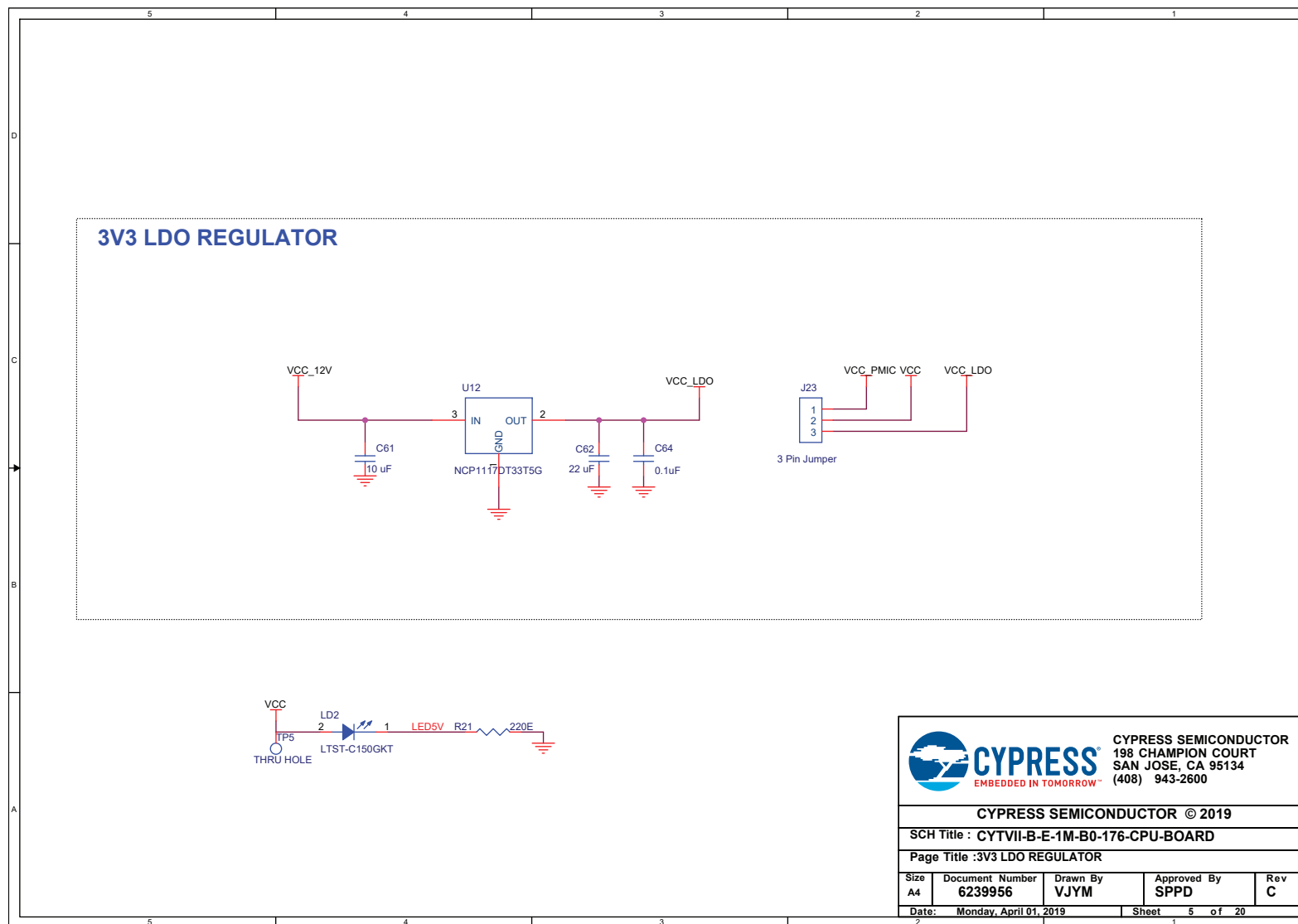
Figure A-4. 3V3 LDO Regulator
