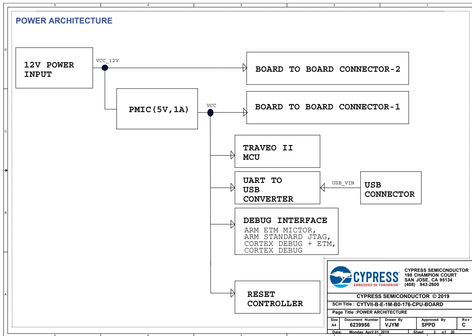
Figure A-2. Power Architecture
