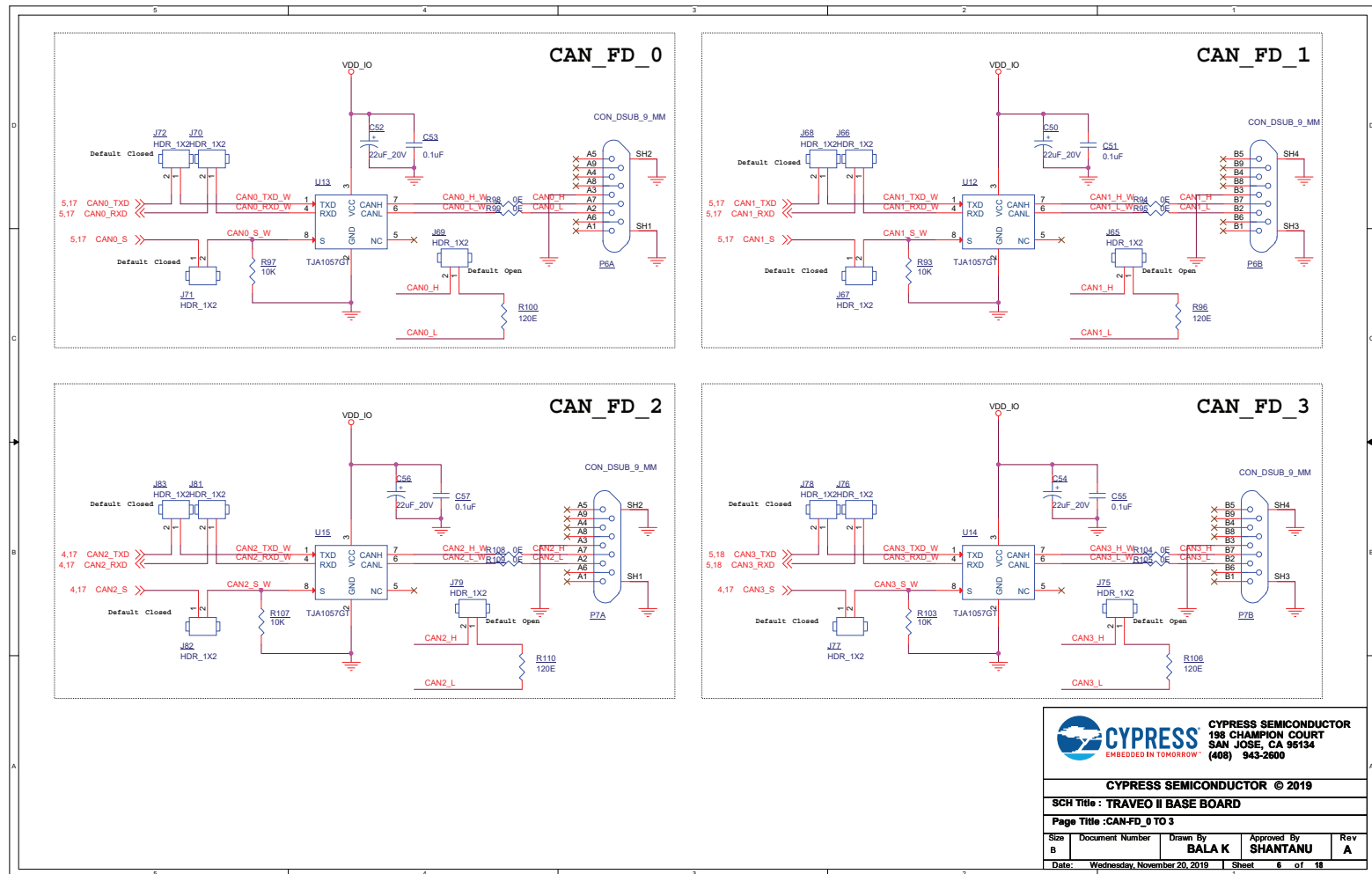
Figure C-4. CAN-FD_0 to 3
