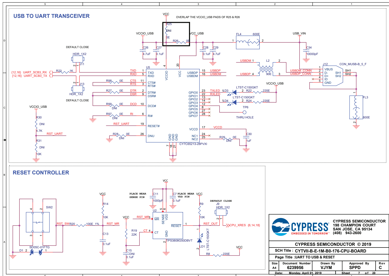
Figure A-6. UART to USB &amp; RESET
