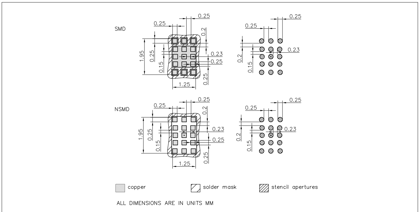
Figure 17 Foot print
