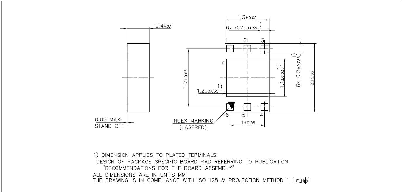
Figure 16 Package outline
