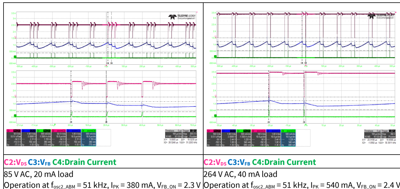
Figure 16 ABM operation
