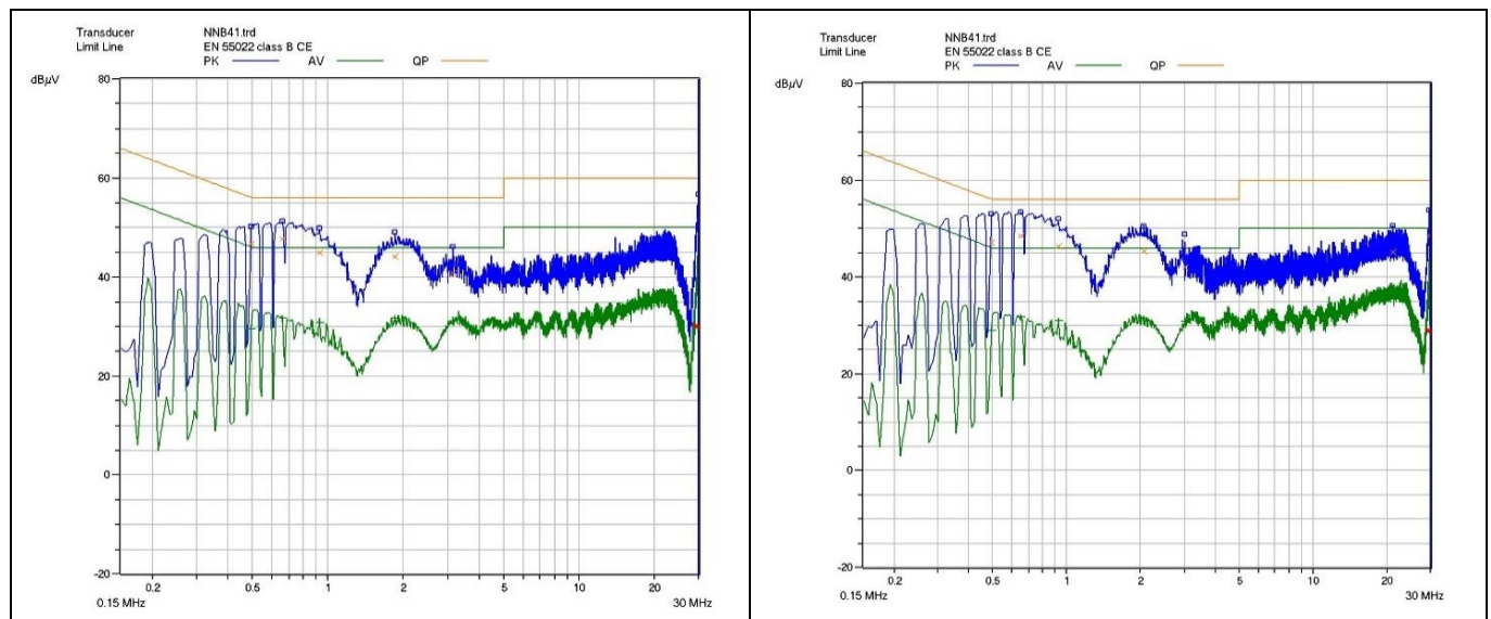
Figure 10 Conducted emissions at 230 V AC with full load
