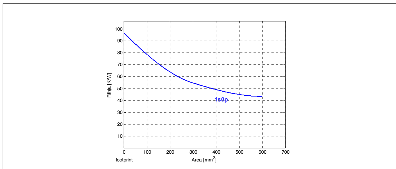
Figure 8 Typical Thermal Resistance. Both channels active. T_a=85^\circ\text{C} . PCB set-up 1s0p
