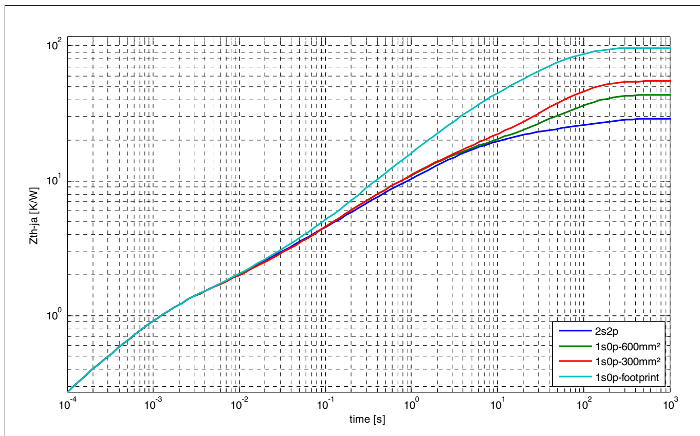
Figure 7 Typical Thermal Impedance. Both channels active. T_a=85^\circ\text{C} . PCB set up according Figure 4 / Figure 5
