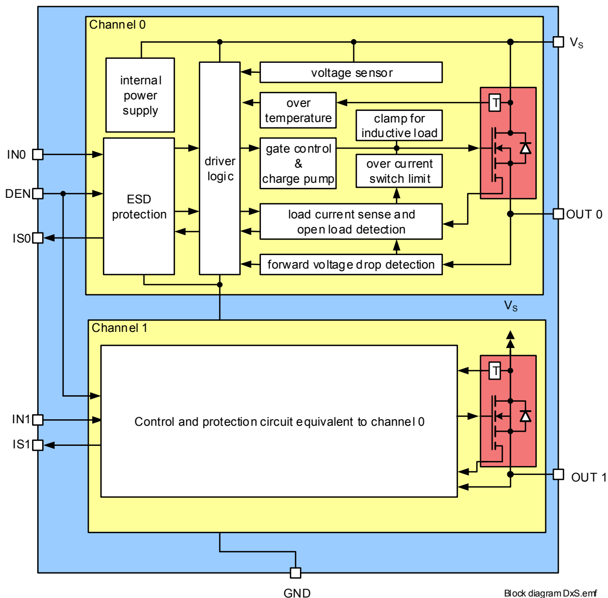
Figure 1 Block Diagram for the BTF6070-2EKV
