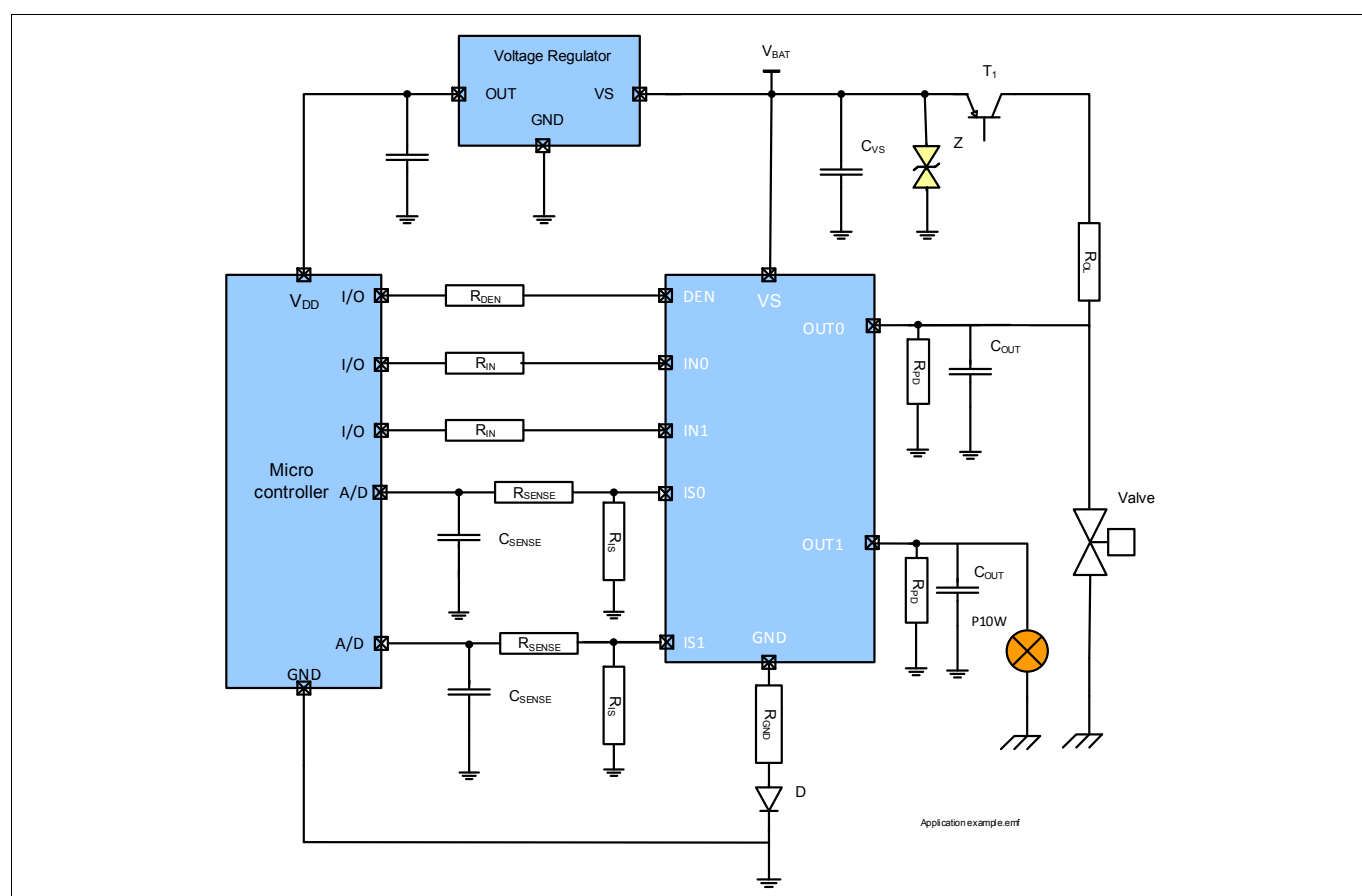
Application Diagram with BTF6070-2EKV
