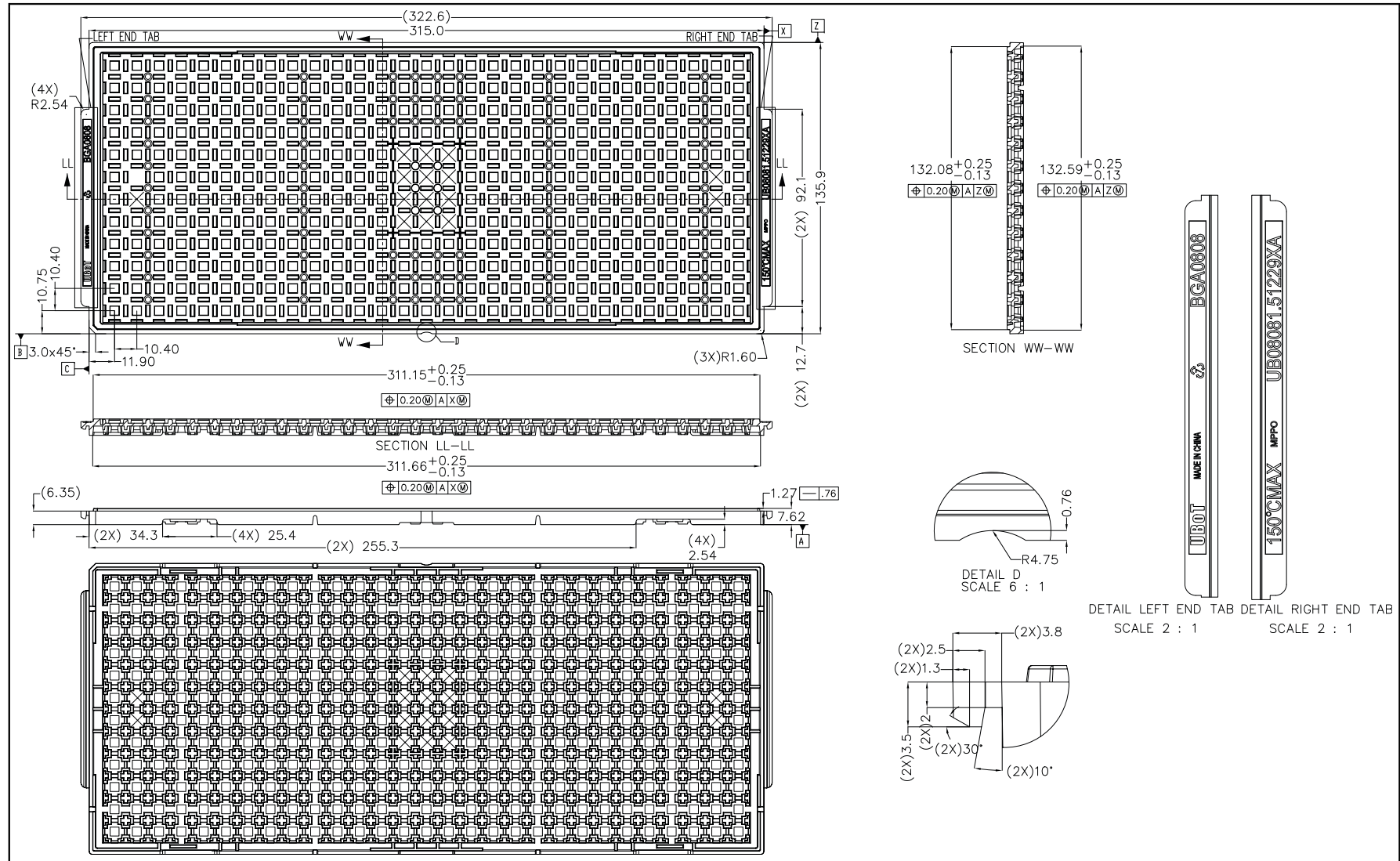
Figure 36: BCM20733 8 × 8 FBGA Package Tray (1 of 2)
