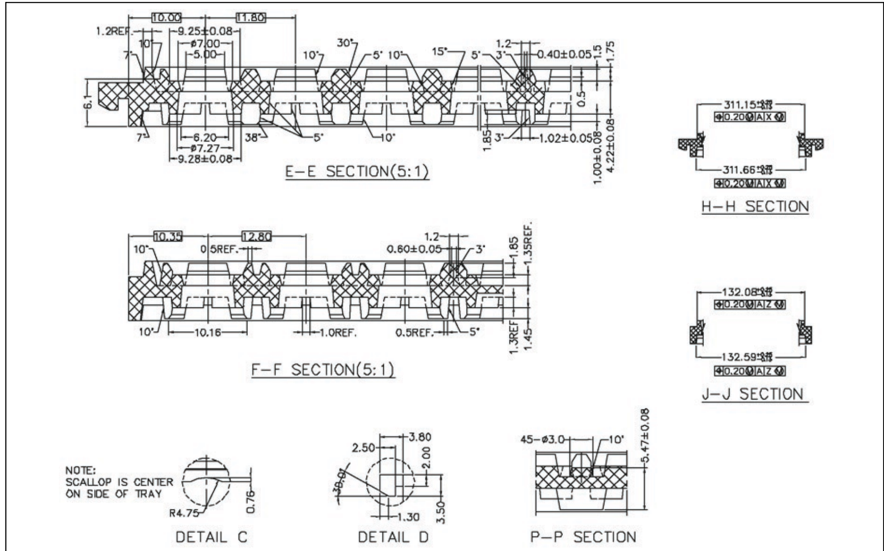
Figure 35: BCM20733 9 × 9 FBGA Package Tray (2 of 2)
