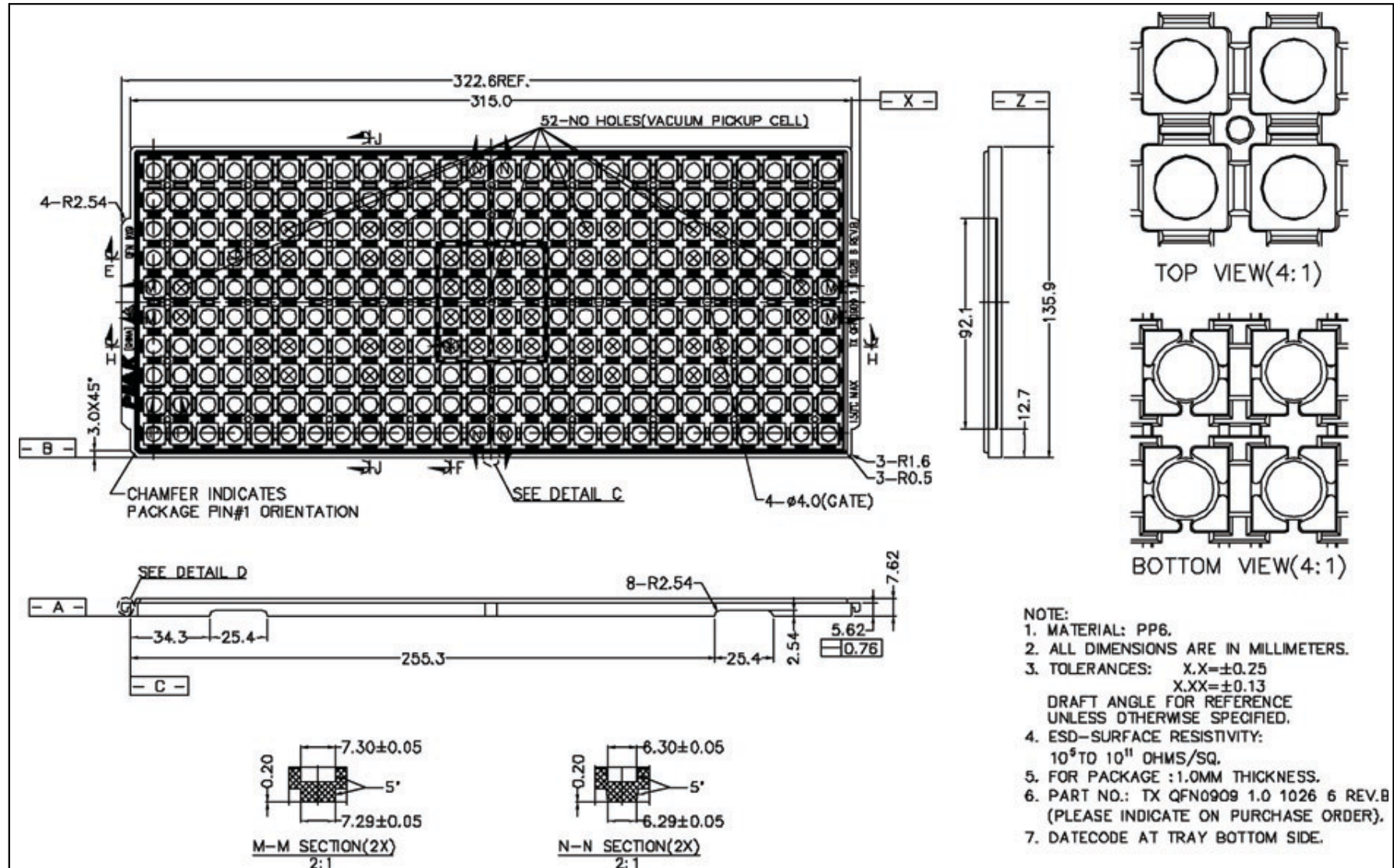
Figure 34: BCM20733 9 × 9 FBGA Package Tray (1 of 2)
