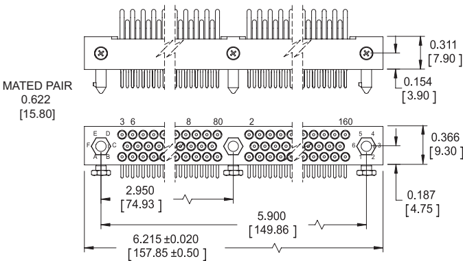
Plug
