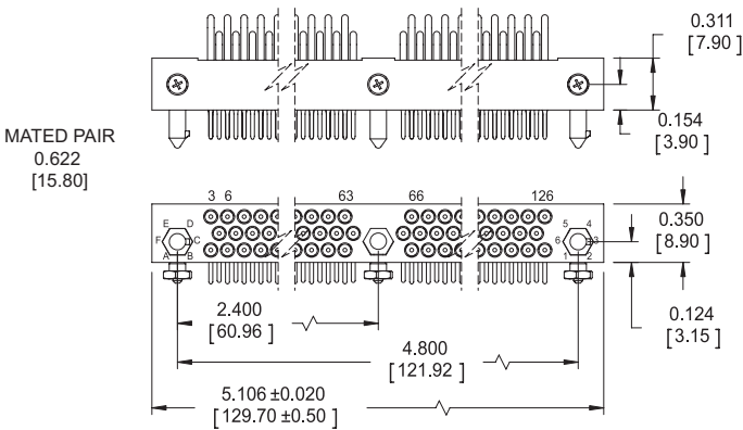
Plug
