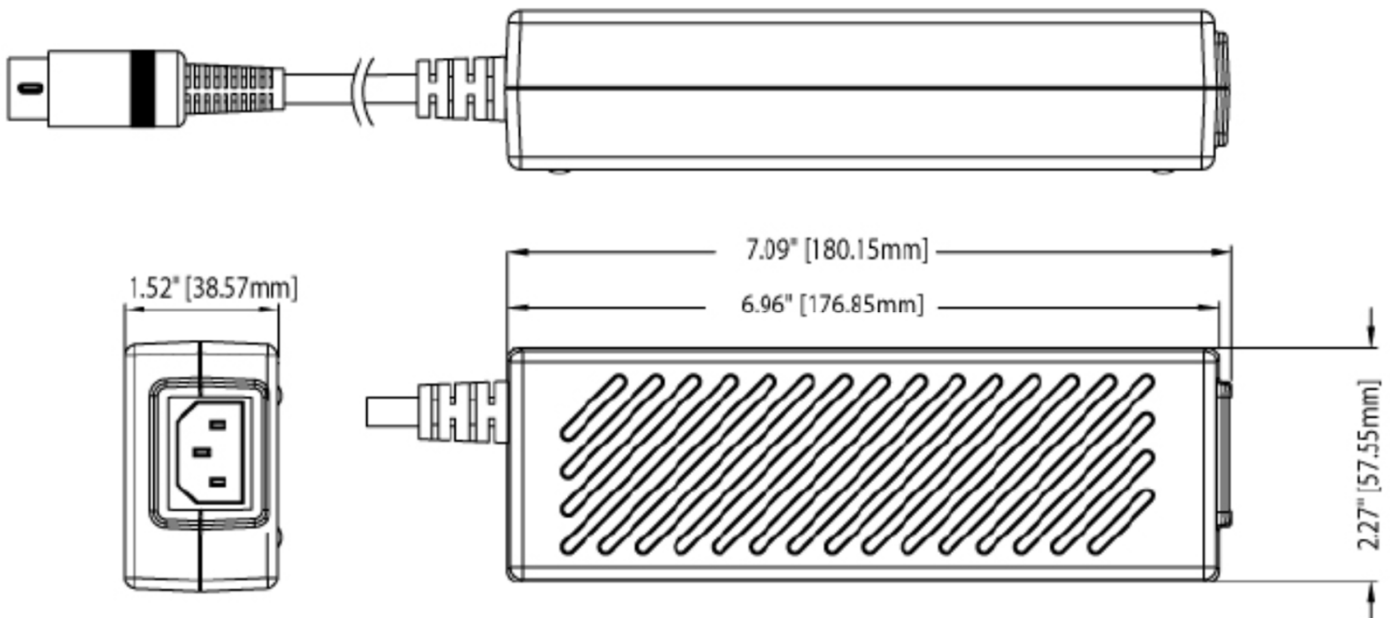
FWC100-Class I-DWG
