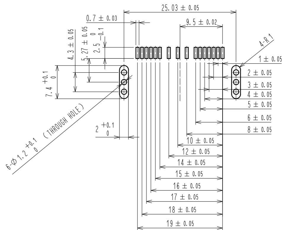
RECOMMENDED PC BOARD PATTERN (CONNECTOR SIDE)
