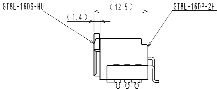
MATED CONNECOTORS
