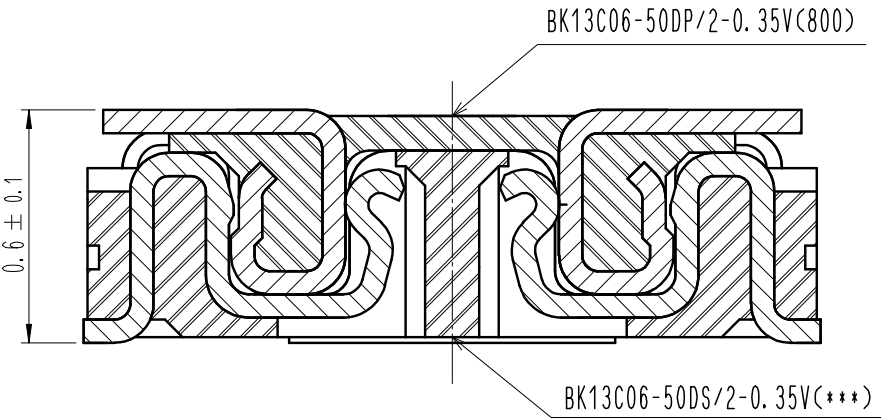
SIGNAL CONTACT
