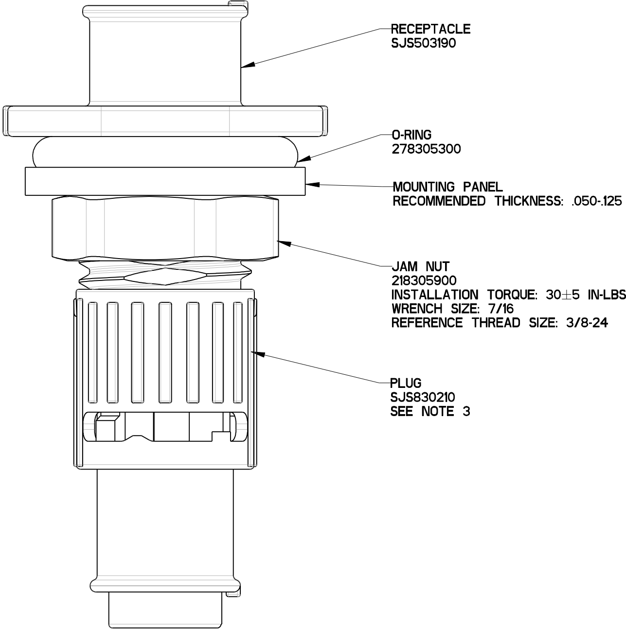
MOUNTING INSTRUCTIONS
