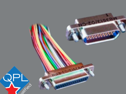
MIL-DTL-83513 Micro-D connectors and accessories
