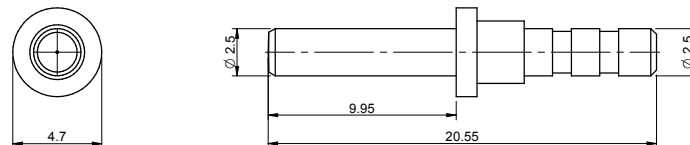
Male Contact
