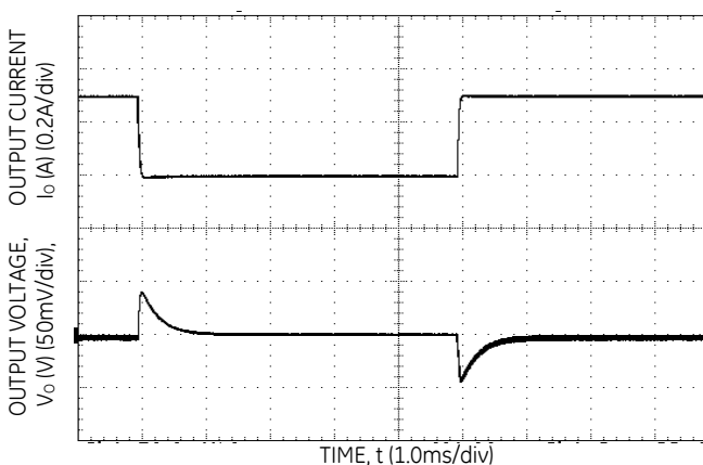
Figure 17. Transient Response to Dynamic Load Change from 50% to 75% to 50% of full load.
