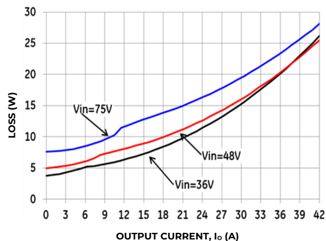
Figure 2. Typical Converter Loss vs. Output Current.
