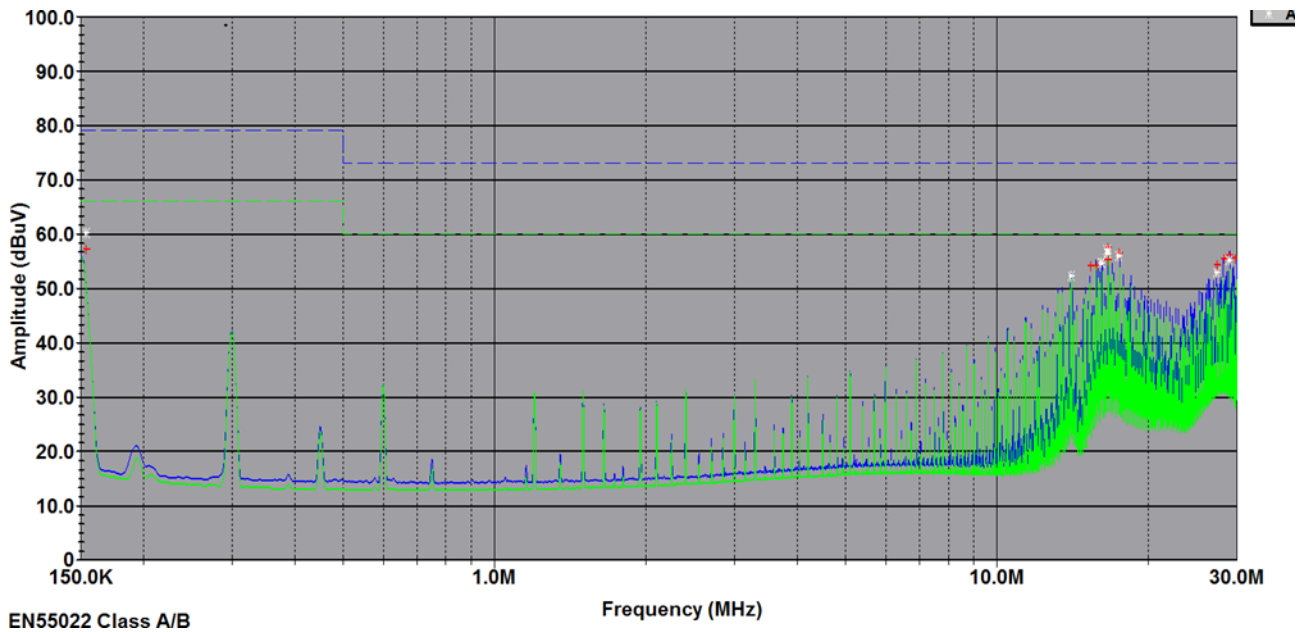
Figure 24. EMC Consideration
