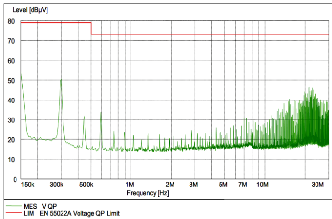
Figure 26. EMC Considerations
