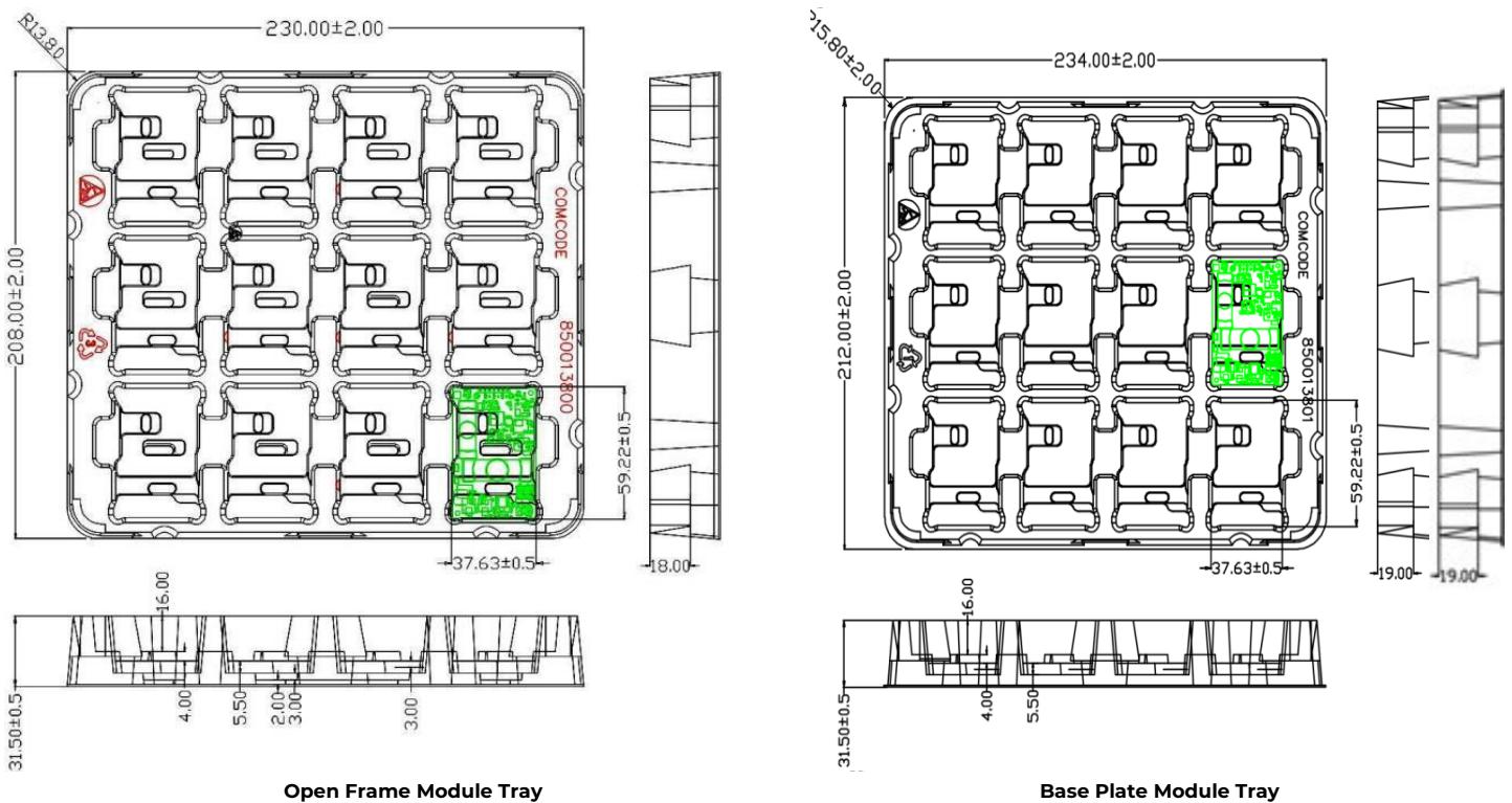
Figure 27. QBVEW033A0B Packaging Tray
