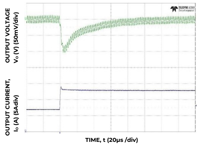
Figure 34 Transient Response to Dynamic Load Change from 50% to 100% at 12V in , C out =8x47µF, C Tune =470pF, R Tune =300Ω
