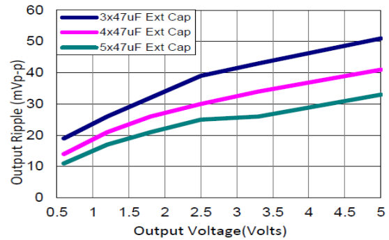
Figure 38. Output ripple voltage for various output voltages with external 3x47 \mu\text{F} , 4x47 \mu\text{F} or 5x47 \mu\text{F} ceramic capacitors at the output (14A load). Input voltage is 12V.
