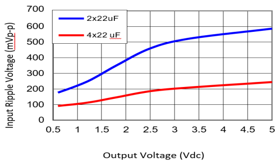
Figure 37. Input ripple voltage for various output voltages with 2x22 \mu\text{F} or 4x22 \mu\text{F} ceramic capacitors at the input (14A load). Input voltage is 12V.
