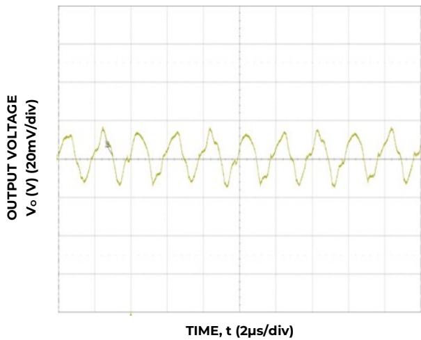
Figure 27. Typical output ripple and noise ( C_o=5x22\mu F ceramic, V_{IN}=12V , I_o = I_{o,max} ).
