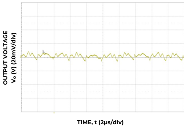
Figure 3. Typical output ripple ( C_o=5x22\mu F ceramic, V_{IN} = 12V , I_o = I_{o,max} ).
