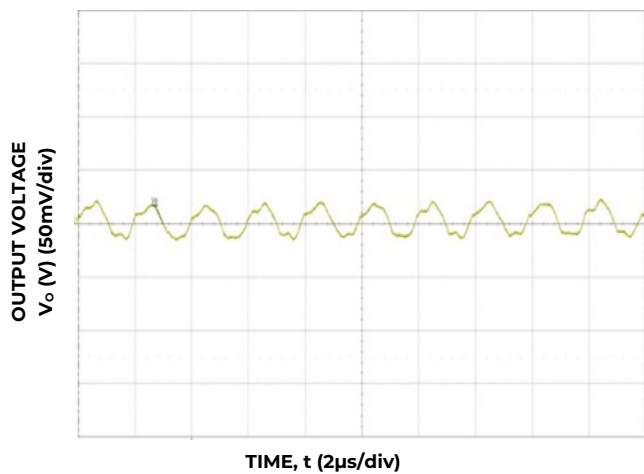
Figure 33. Typical output ripple and noise (C o =5x22µF ceramic, V IN = 12V, I o = I o,max .)
