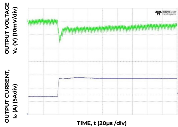
Figure 4. Transient Response to Dynamic Load Change from 50% to 100% at 12Vin, C_{out}=8x47\mu F+8x330\mu F C_{Tune}=27nF , R_{Tune}=300\Omega
