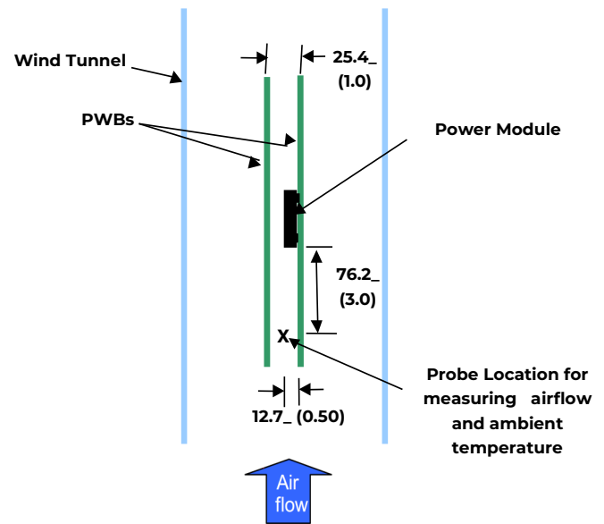
Figure 48. Thermal Test Setup.
