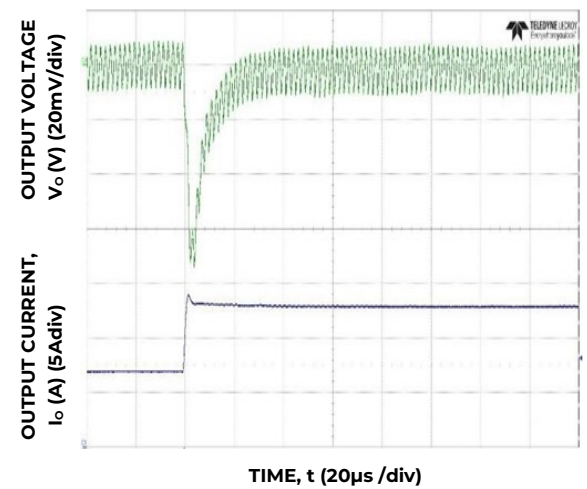
Figure 28 Transient Response to Dynamic Load Change from 50% to 100% at 12Vin, C_{out}=8x47\mu F , C_{Tune}=1.2nF , R_{Tune}=300\Omega
