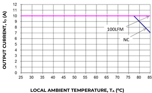
Figure 14. Output Current Derating for the Open Frame KSTW010A0F in the Transverse Orientation; Airflow from V_{in}(+) to V_{in}(-) ; V_{in} = 48V .
