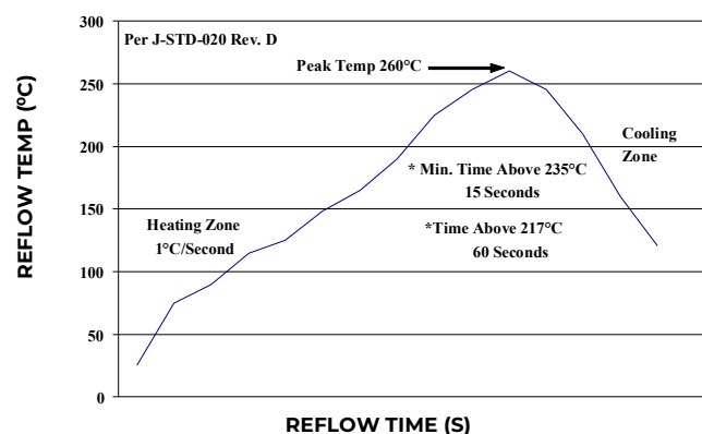
Figure 21. Recommended linear reflow profile using Sn/Ag/Cu solder.
