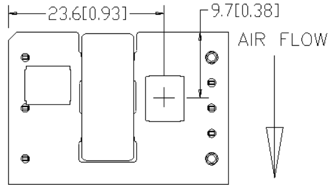
Figure 15. T_{ref} Temperature Measurement Location.
