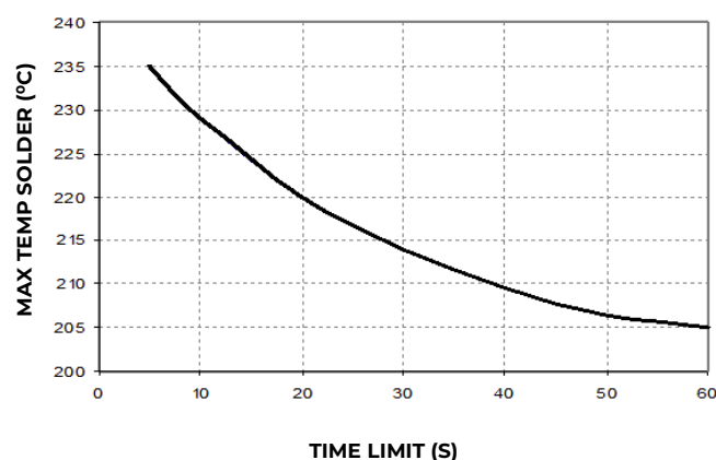
Figure 20. Time Limit, T_{lim} , Curve Above 205°C Reflow.
