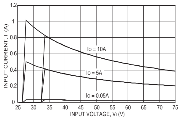
Figure 19. Input Voltage and Current Characteristics.
