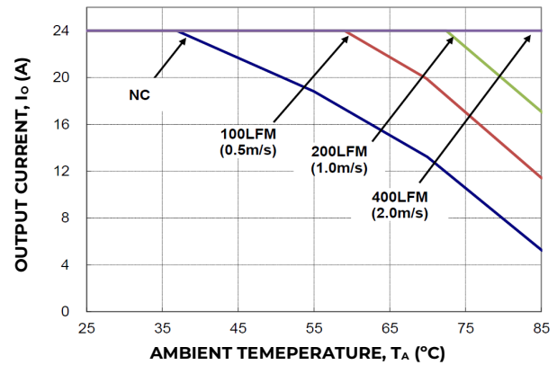
Figure 16. Output Current Derating for the Module with Heatplate; Airflow in the Transverse Direction from V_{out}(-) to V_{out}(+) ; V_{IN}=48V , V_O=5.0V .
